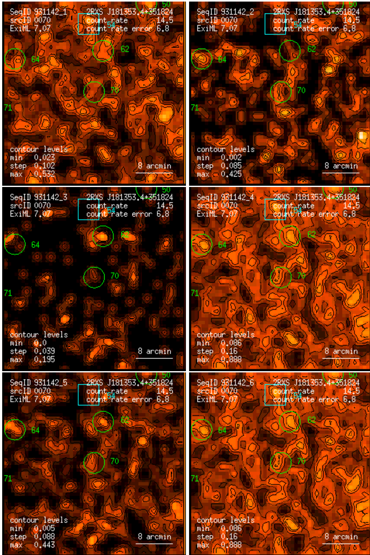
Figure 70: RASS 931142: detection 0070: band rate images, Gaussian filter: (1) PSPC channels 11 – 41, (2) 52 – 90, (3) 91 – 201, (4) 11 – 235, (5) 52 – 201, (6) 11 – 201. Broad band rates in counts/ks. Band rate contour levels in counts/ks/arcmin 2 .
