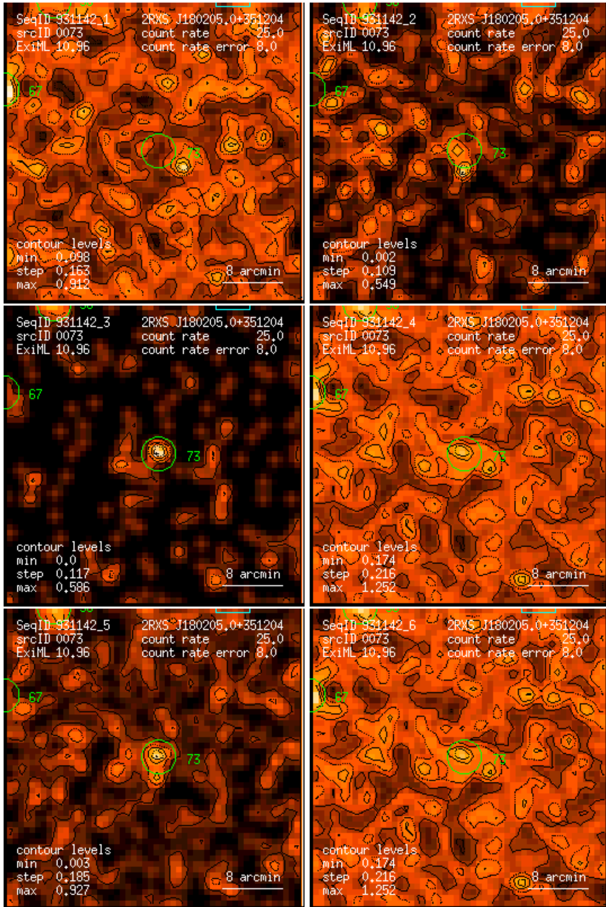
Figure 73: RASS 931142: detection 0073: band rate images, Gaussian filter: (1) PSPC channels 11 – 41, (2) 52 – 90, (3) 91 – 201, (4) 11 – 235, (5) 52 – 201, (6) 11 – 201. Broad band rates in counts/ks. Band rate contour levels in counts/ks/arcmin 2 .
