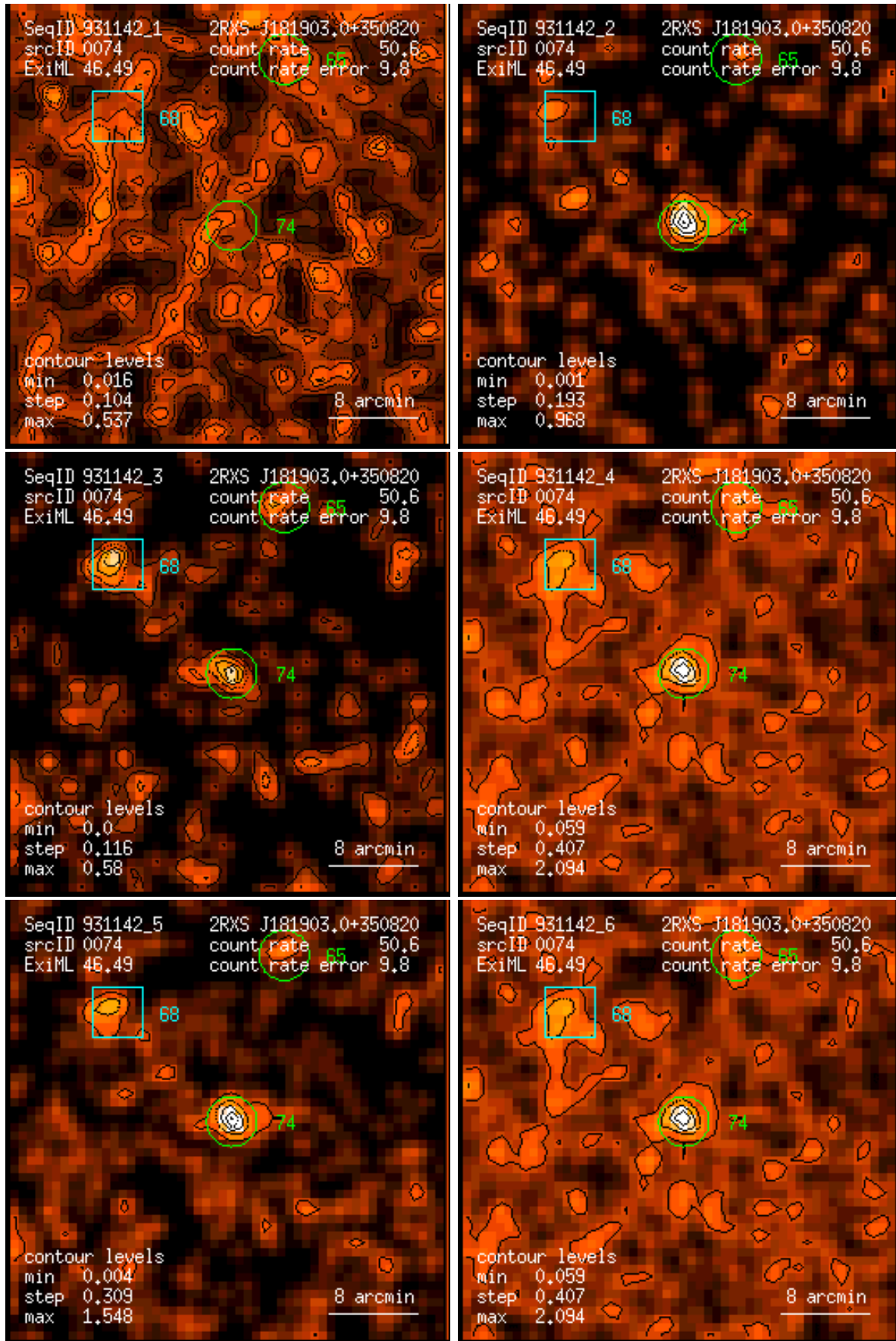
Figure 74: RASS 931142: detection 0074: band rate images, Gaussian filter: (1) PSPC channels 11 – 41, (2) 52 – 90, (3) 91 – 201, (4) 11 – 235, (5) 52 – 201, (6) 11 – 201. Broad band rates in counts/ks. Band rate contour levels in counts/ks/arcmin 2 .
