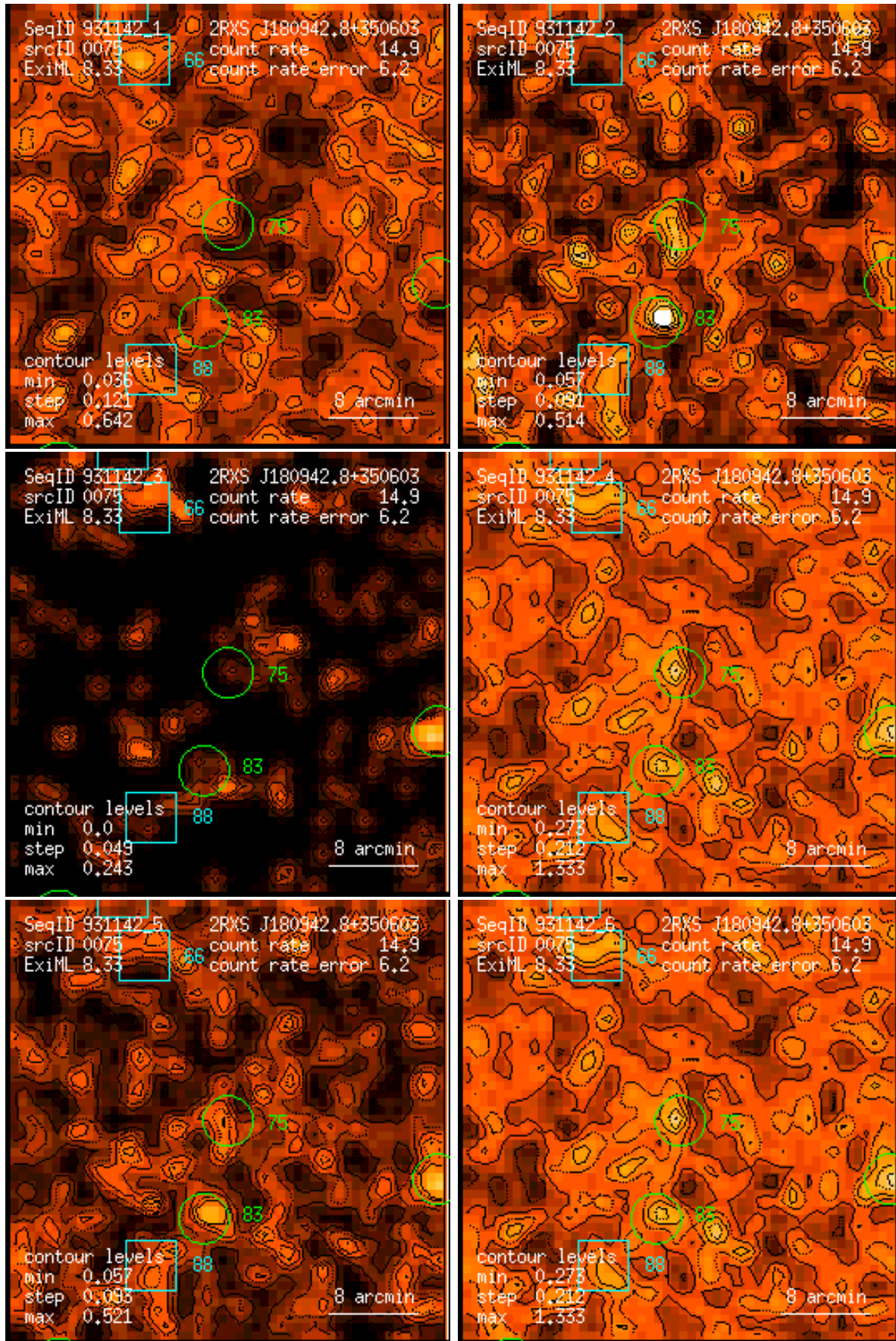
Figure 75: RASS 931142: detection 0075: band rate images, Gaussian filter: (1) PSPC channels 11 – 41, (2) 52 – 90, (3) 91 – 201, (4) 11 – 235, (5) 52 – 201, (6) 11 – 201. Broad band rates in counts/ks. Band rate contour levels in counts/ks/arcmin 2 .
