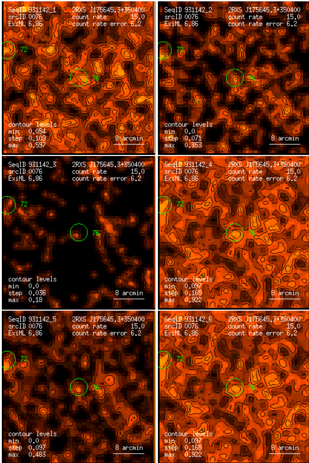
Figure 76: RASS 931142: detection 0076: band rate images, Gaussian filter: (1) PSPC channels 11 – 41, (2) 52 – 90, (3) 91 – 201, (4) 11 – 235, (5) 52 – 201, (6) 11 – 201. Broad band rates in counts/ks. Band rate contour levels in counts/ks/arcmin 2 .
