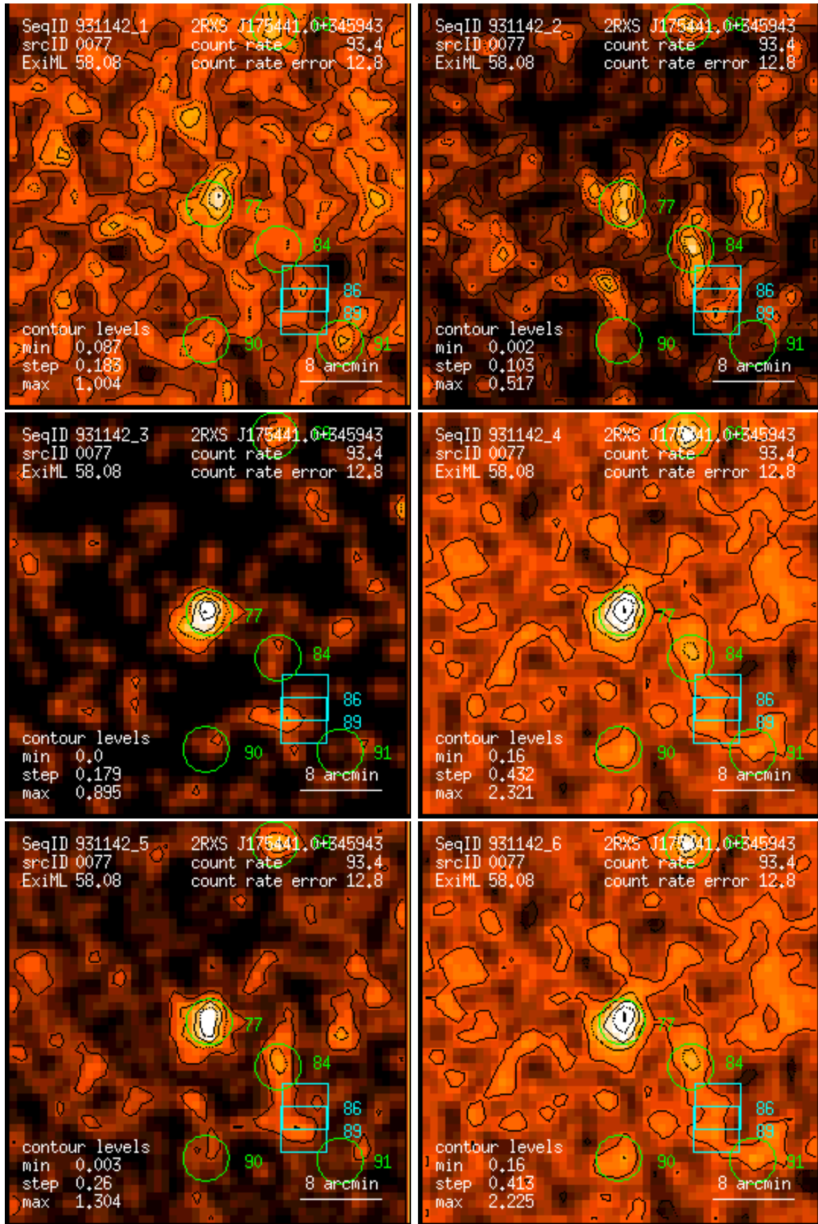
Figure 77: RASS 931142: detection 0077: band rate images, Gaussian filter: (1) PSPC channels 11 – 41, (2) 52 – 90, (3) 91 – 201, (4) 11 – 235, (5) 52 – 201, (6) 11 – 201. Broad band rates in counts/ks. Band rate contour levels in counts/ks/arcmin 2 .
