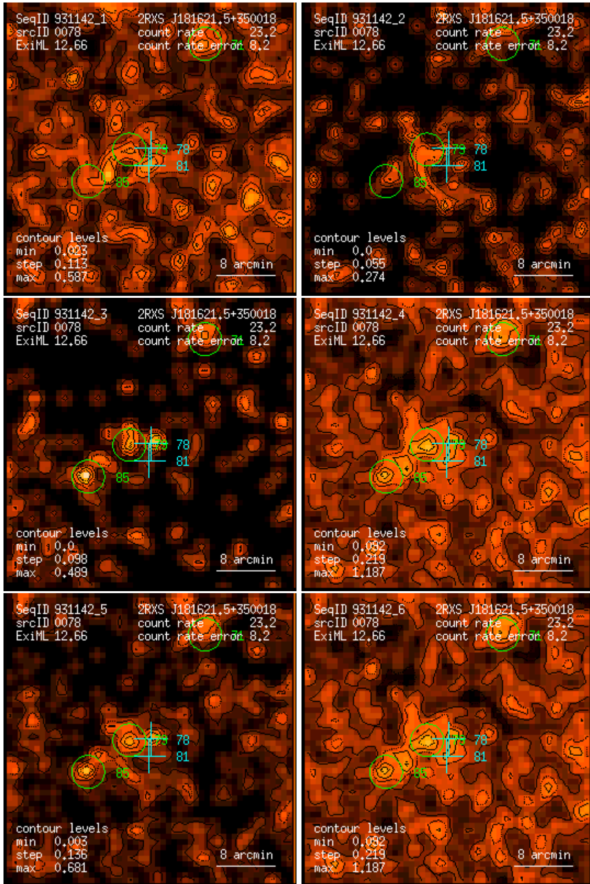
Figure 78: RASS 931142: detection 0078: band rate images, Gaussian filter: (1) PSPC channels 11 – 41, (2) 52 – 90, (3) 91 – 201, (4) 11 – 235, (5) 52 – 201, (6) 11 – 201. Broad band rates in counts/ks. Band rate contour levels in counts/ks/arcmin 2 .
