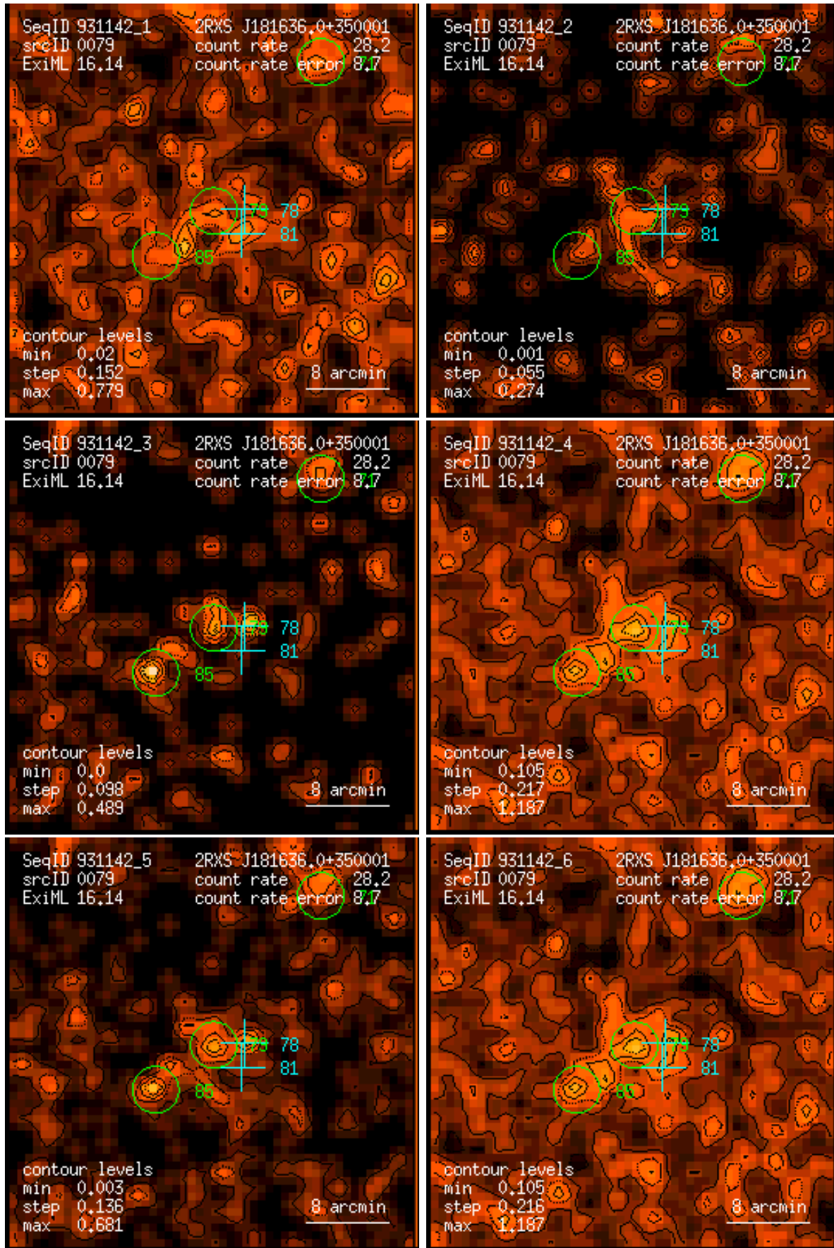
Figure 79: RASS 931142: detection 0079: band rate images, Gaussian filter: (1) PSPC channels 11 – 41, (2) 52 – 90, (3) 91 – 201, (4) 11 – 235, (5) 52 – 201, (6) 11 – 201. Broad band rates in counts/ks. Band rate contour levels in counts/ks/arcmin 2 .
