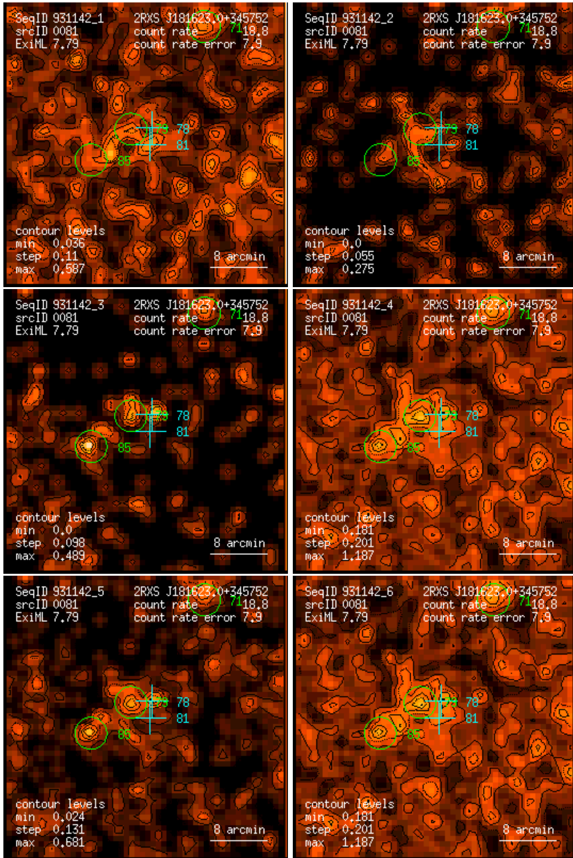
Figure 81: RASS 931142: detection 0081: band rate images, Gaussian filter: (1) PSPC channels 11 – 41, (2) 52 – 90, (3) 91 – 201, (4) 11 – 235, (5) 52 – 201, (6) 11 – 201. Broad band rates in counts/ks. Band rate contour levels in counts/ks/arcmin 2 .
