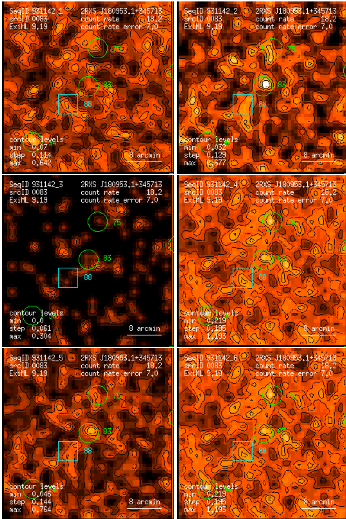
Figure 83: RASS 931142: detection 0083: band rate images, Gaussian filter: (1) PSPC channels 11 – 41, (2) 52 – 90, (3) 91 – 201, (4) 11 – 235, (5) 52 – 201, (6) 11 – 201. Broad band rates in counts/ks. Band rate contour levels in counts/ks/arcmin 2 .
