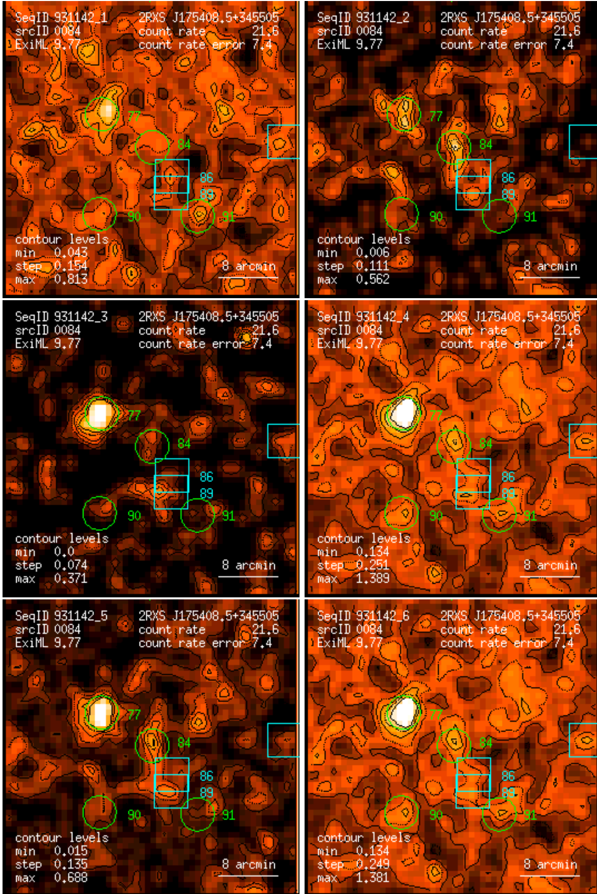
Figure 84: RASS 931142: detection 0084: band rate images, Gaussian filter: (1) PSPC channels 11 – 41, (2) 52 – 90, (3) 91 – 201, (4) 11 – 235, (5) 52 – 201, (6) 11 – 201. Broad band rates in counts/ks. Band rate contour levels in counts/ks/arcmin 2 .
