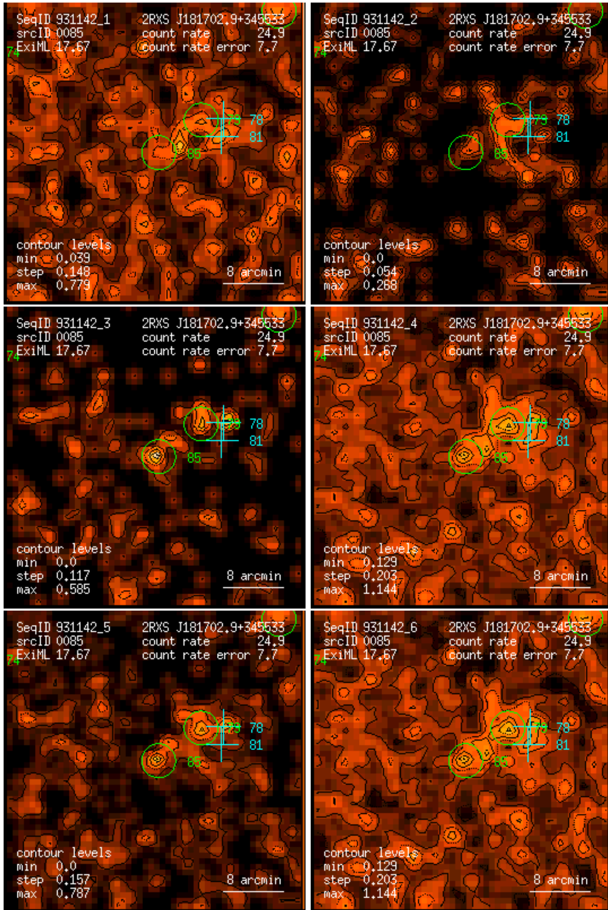
Figure 85: RASS 931142: detection 0085: band rate images, Gaussian filter: (1) PSPC channels 11 – 41, (2) 52 – 90, (3) 91 – 201, (4) 11 – 235, (5) 52 – 201, (6) 11 – 201. Broad band rates in counts/ks. Band rate contour levels in counts/ks/arcmin 2 .
