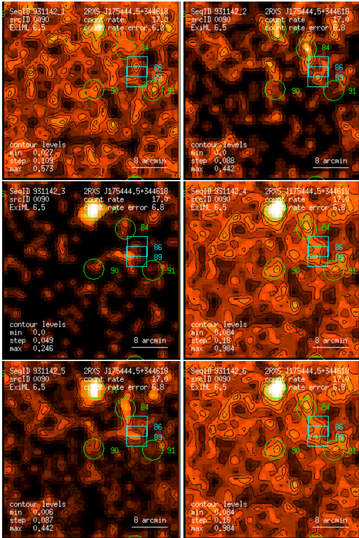
Figure 90: RASS 931142: detection 0090: band rate images, Gaussian filter: (1) PSPC channels 11 – 41, (2) 52 – 90, (3) 91 – 201, (4) 11 – 235, (5) 52 – 201, (6) 11 – 201. Broad band rates in counts/ks. Band rate contour levels in counts/ks/arcmin 2 .
