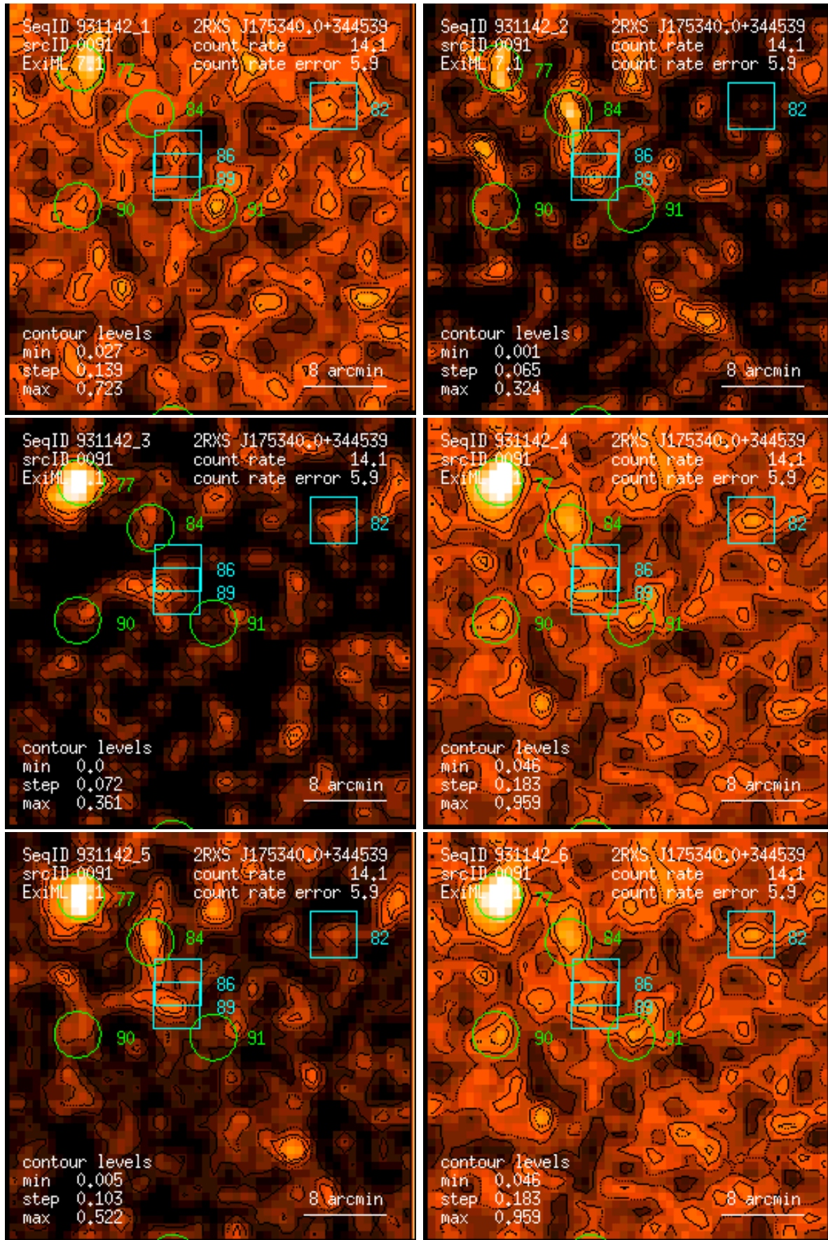
Figure 91: RASS 931142: detection 0091: band rate images, Gaussian filter: (1) PSPC channels 11 – 41, (2) 52 – 90, (3) 91 – 201, (4) 11 – 235, (5) 52 – 201, (6) 11 – 201. Broad band rates in counts/ks. Band rate contour levels in counts/ks/arcmin 2 .
