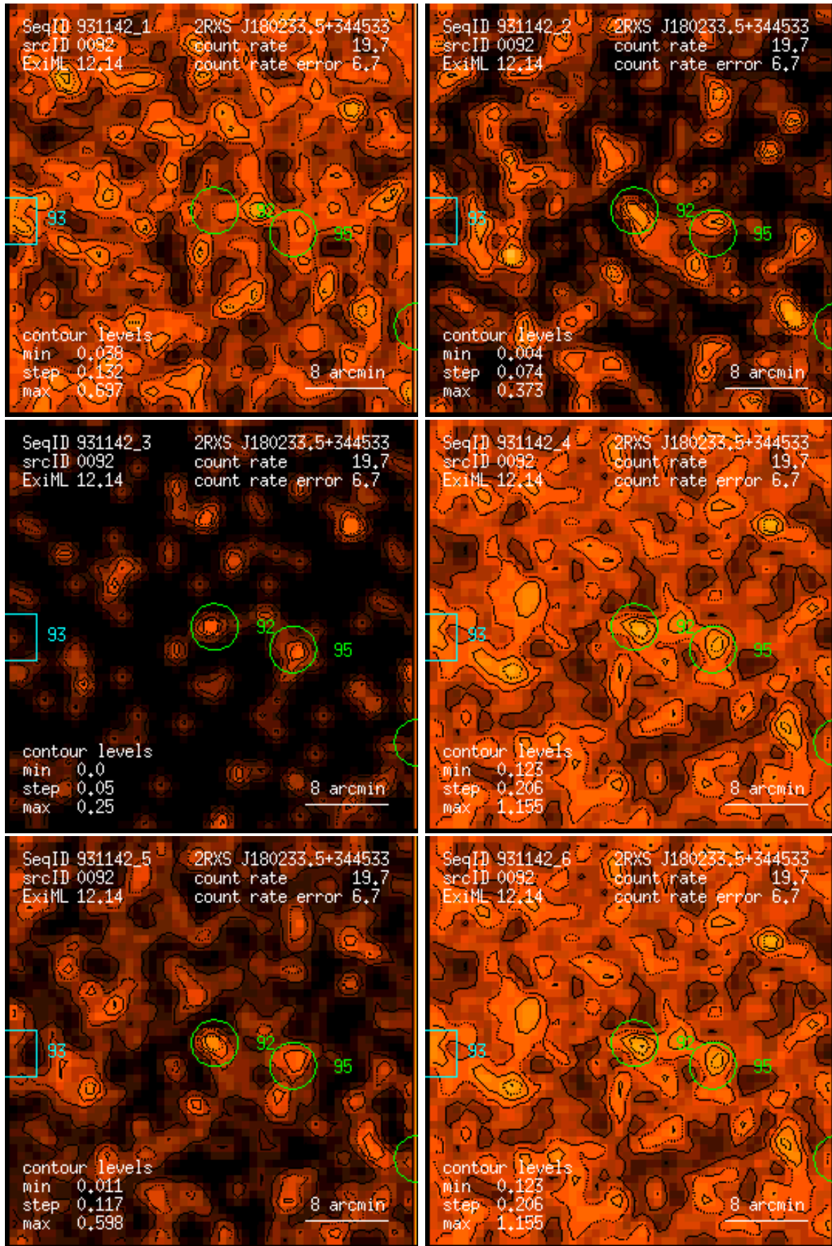
Figure 92: RASS 931142: detection 0092: band rate images, Gaussian filter: (1) PSPC channels 11 – 41, (2) 52 – 90, (3) 91 – 201, (4) 11 – 235, (5) 52 – 201, (6) 11 – 201. Broad band rates in counts/ks. Band rate contour levels in counts/ks/arcmin 2 .
