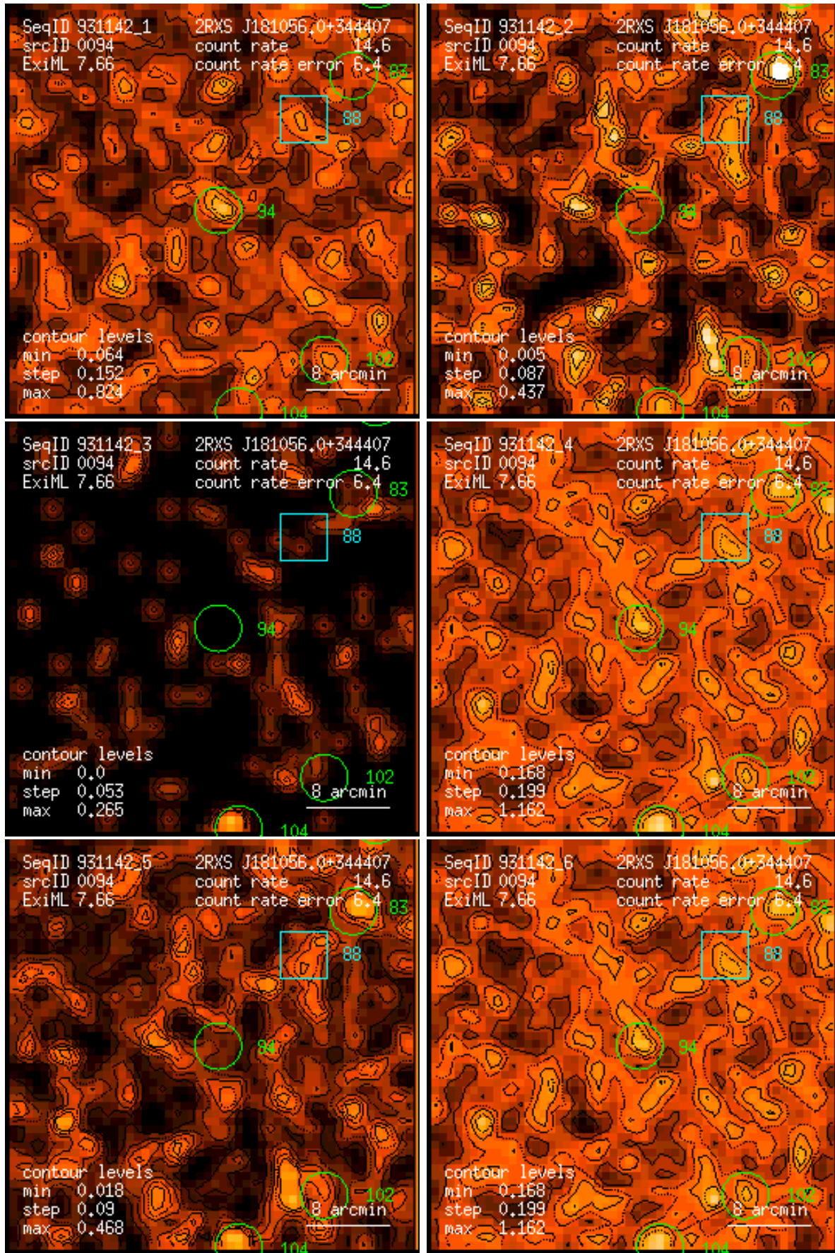
Figure 94: RASS 931142: detection 0094: band rate images, Gaussian filter: (1) PSPC channels 11 – 41, (2) 52 – 90, (3) 91 – 201, (4) 11 – 235, (5) 52 – 201, (6) 11 – 201. Broad band rates in counts/ks. Band rate contour levels in counts/ks/arcmin 2 .
