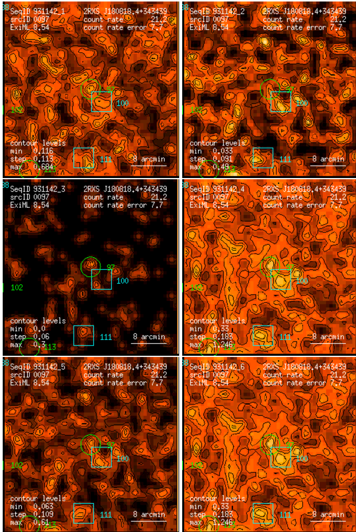
Figure 97: RASS 931142: detection 0097: band rate images, Gaussian filter: (1) PSPC channels 11 – 41, (2) 52 – 90, (3) 91 – 201, (4) 11 – 235, (5) 52 – 201, (6) 11 – 201. Broad band rates in counts/ks. Band rate contour levels in counts/ks/arcmin 2 .
