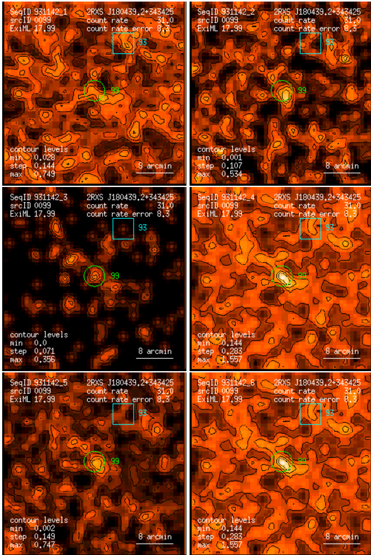
Figure 99: RASS 931142: detection 0099: band rate images, Gaussian filter: (1) PSPC channels 11 – 41, (2) 52 – 90, (3) 91 – 201, (4) 11 – 235, (5) 52 – 201, (6) 11 – 201. Broad band rates in counts/ks. Band rate contour levels in counts/ks/arcmin 2 .
