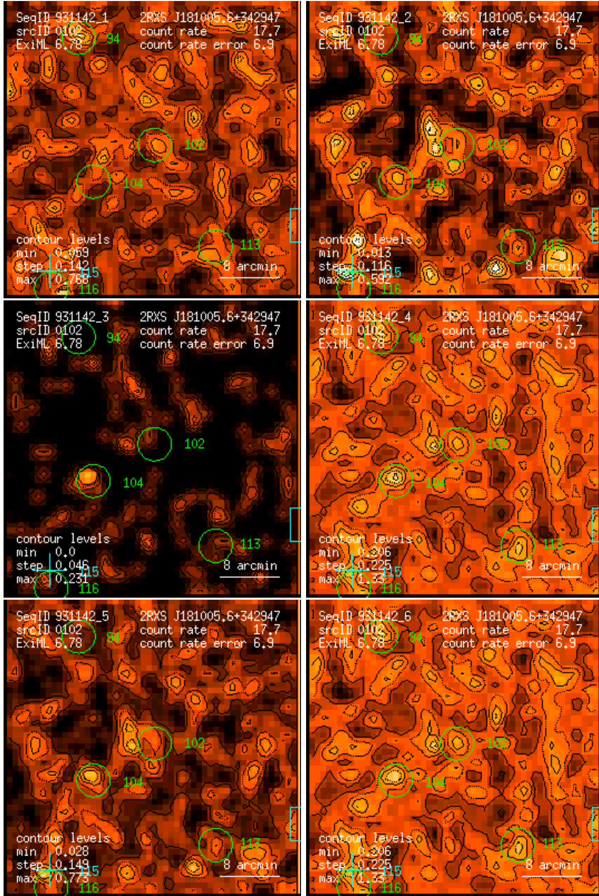
Figure 102: RASS 931142: detection 0102: band rate images, Gaussian filter: (1) PSPC channels 11 – 41, (2) 52 – 90, (3) 91 – 201, (4) 11 – 235, (5) 52 – 201, (6) 11 – 201. Broad band rates in counts/ks. Band rate contour levels in counts/ks/arcmin 2 .
