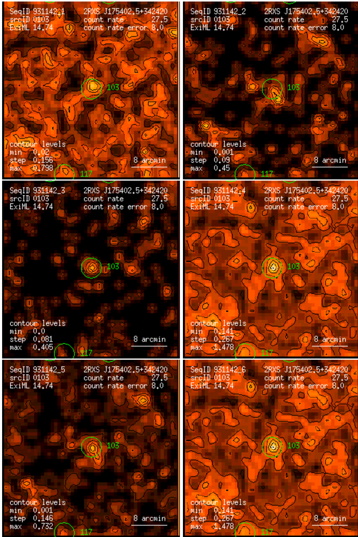
Figure 103: RASS 931142: detection 0103: band rate images, Gaussian filter: (1) PSPC channels 11 – 41, (2) 52 – 90, (3) 91 – 201, (4) 11 – 235, (5) 52 – 201, (6) 11 – 201. Broad band rates in counts/ks. Band rate contour levels in counts/ks/arcmin 2 .
