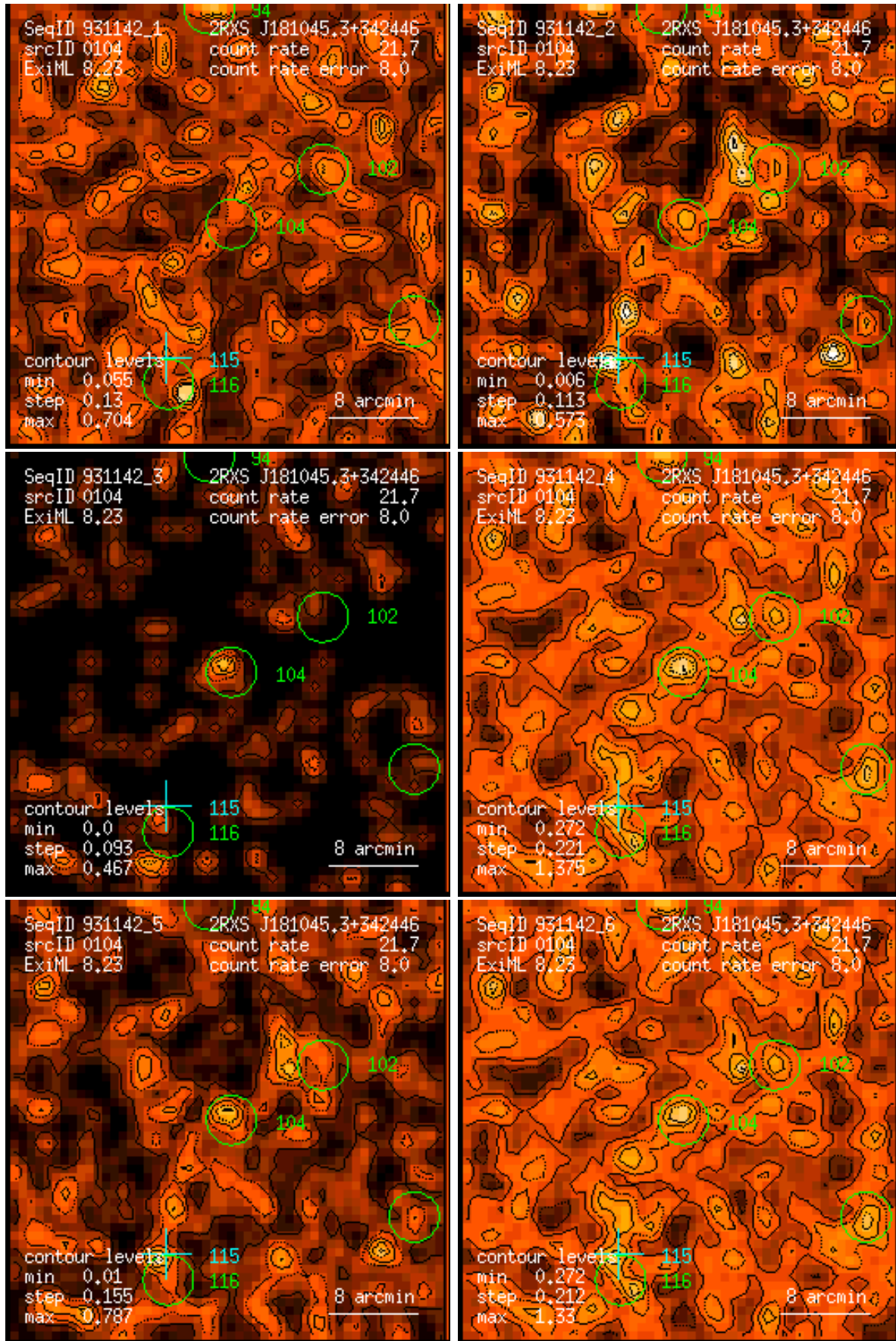
Figure 104: RASS 931142: detection 0104: band rate images, Gaussian filter: (1) PSPC channels 11 – 41, (2) 52 – 90, (3) 91 – 201, (4) 11 – 235, (5) 52 – 201, (6) 11 – 201. Broad band rates in counts/ks. Band rate contour levels in counts/ks/arcmin 2 .
