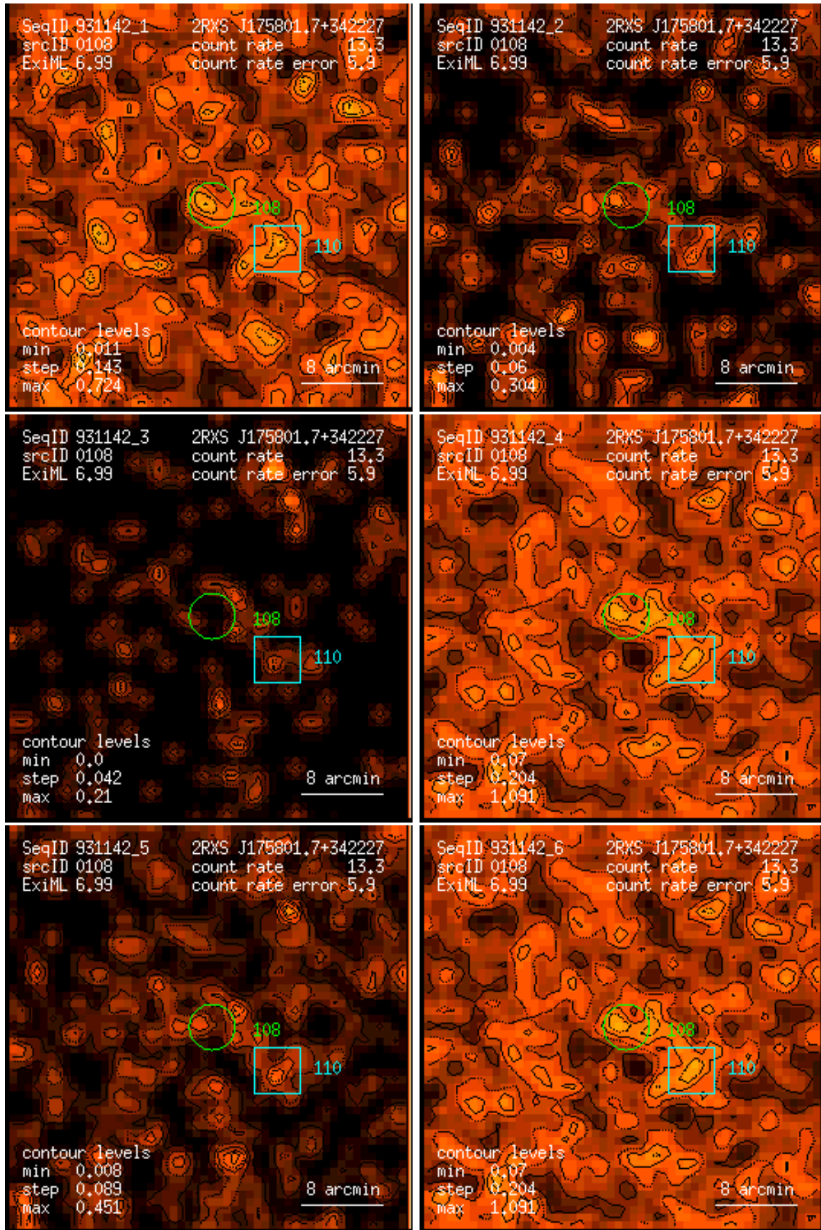
Figure 108: RASS 931142: detection 0108: band rate images, Gaussian filter: (1) PSPC channels 11 – 41, (2) 52 – 90, (3) 91 – 201, (4) 11 – 235, (5) 52 – 201, (6) 11 – 201. Broad band rates in counts/ks. Band rate contour levels in counts/ks/arcmin 2 .
