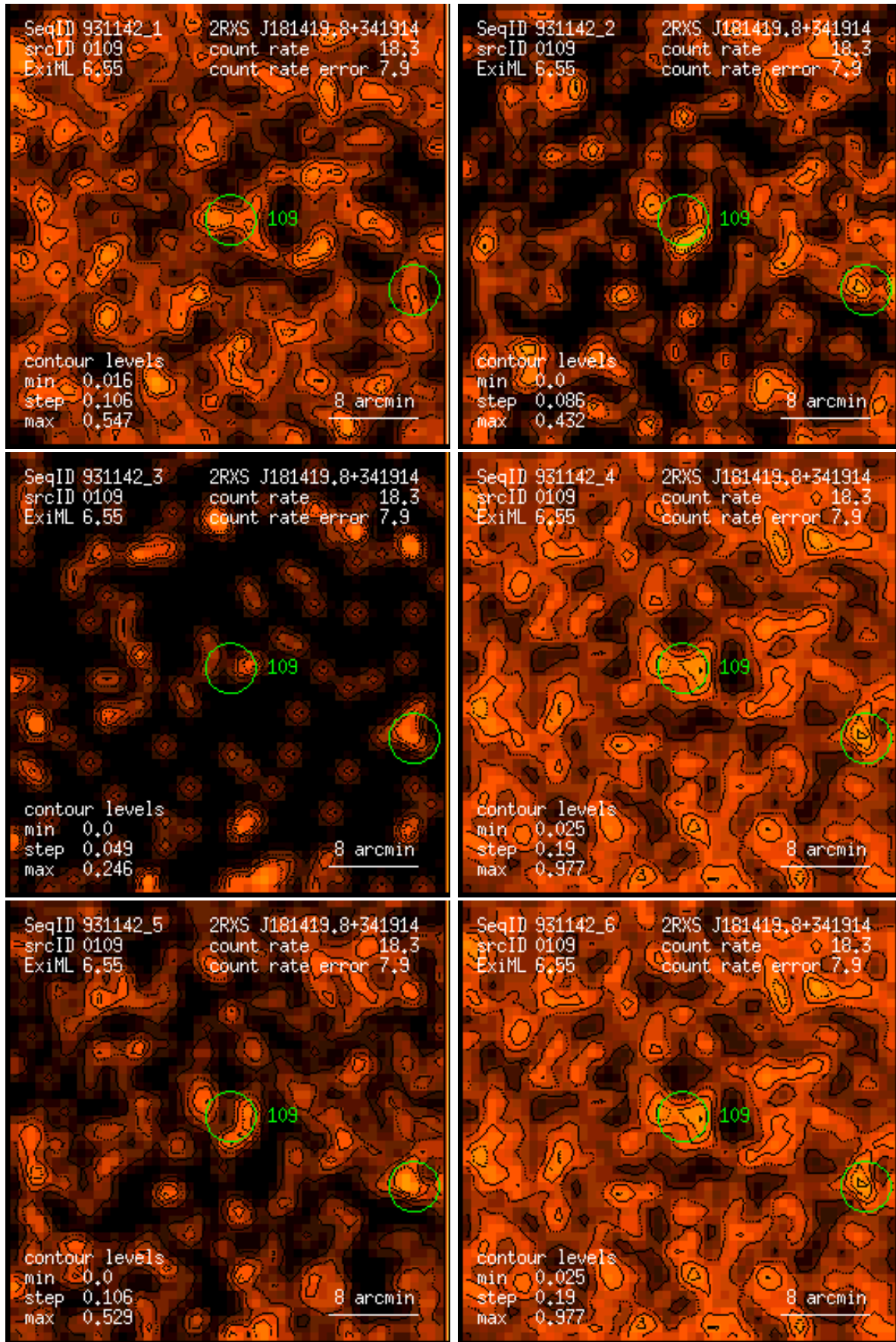
Figure 109: RASS 931142: detection 0109: band rate images, Gaussian filter: (1) PSPC channels 11 – 41, (2) 52 – 90, (3) 91 – 201, (4) 11 – 235, (5) 52 – 201, (6) 11 – 201. Broad band rates in counts/ks. Band rate contour levels in counts/ks/arcmin 2 .
