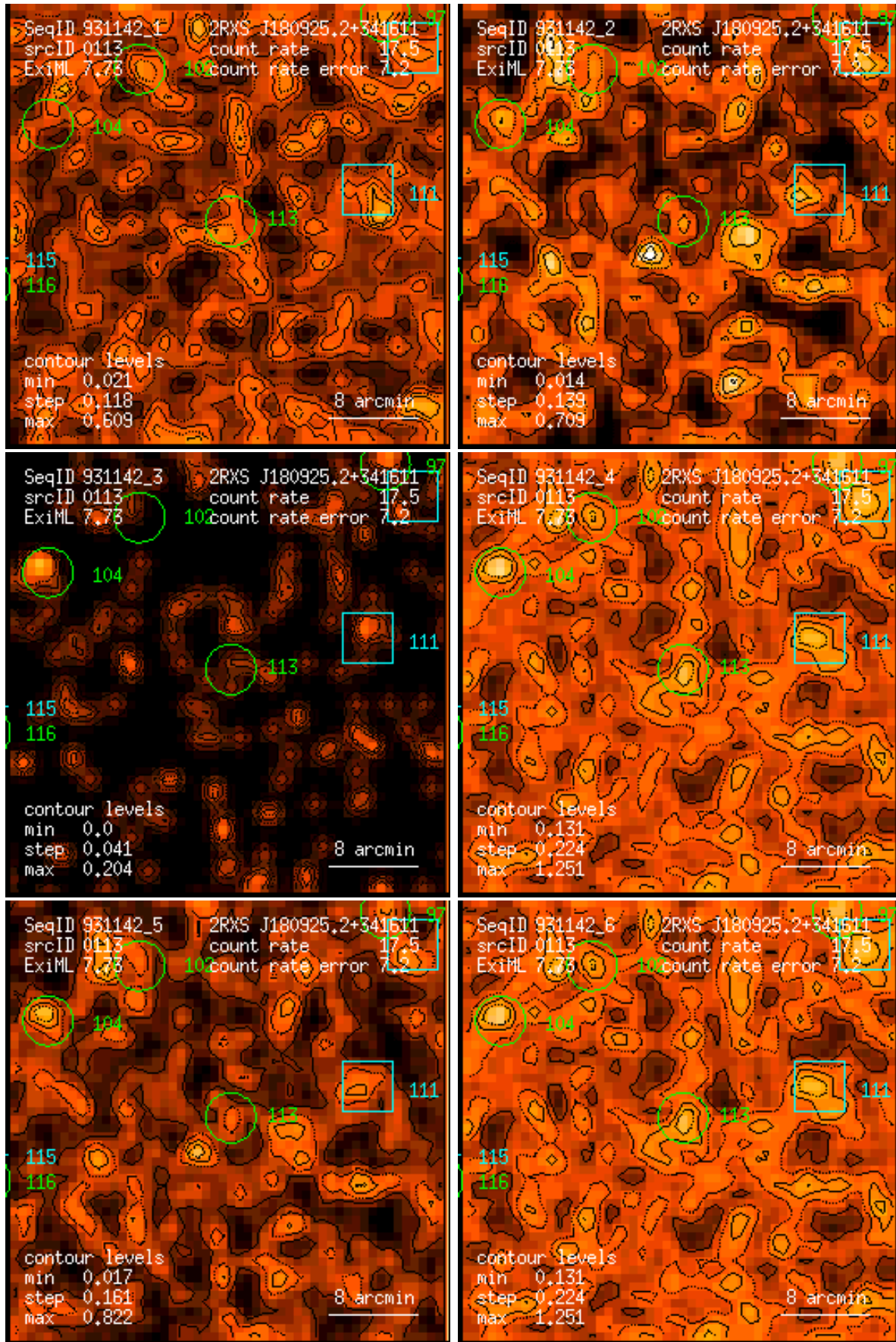
Figure 113: RASS 931142: detection 0113: band rate images, Gaussian filter: (1) PSPC channels 11 – 41, (2) 52 – 90, (3) 91 – 201, (4) 11 – 235, (5) 52 – 201, (6) 11 – 201. Broad band rates in counts/ks. Band rate contour levels in counts/ks/arcmin 2 .
