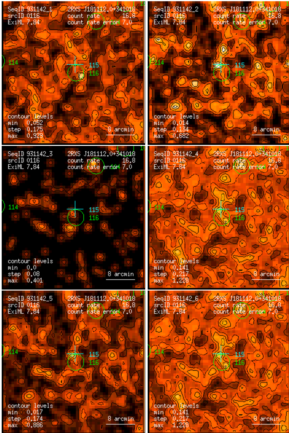
Figure 116: RASS 931142: detection 0116: band rate images, Gaussian filter: (1) PSPC channels 11 – 41, (2) 52 – 90, (3) 91 – 201, (4) 11 – 235, (5) 52 – 201, (6) 11 – 201. Broad band rates in counts/ks. Band rate contour levels in counts/ks/arcmin 2 .
