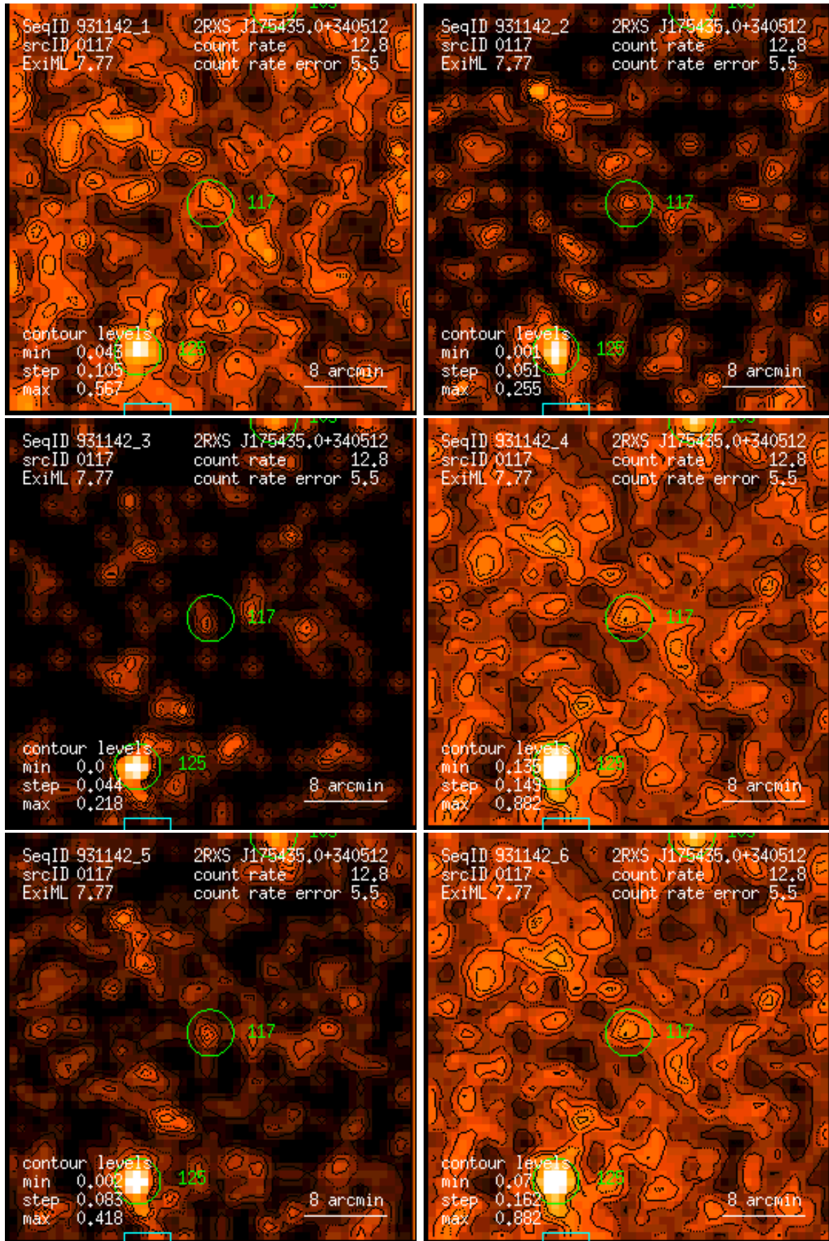
Figure 117: RASS 931142: detection 0117: band rate images, Gaussian filter: (1) PSPC channels 11 – 41, (2) 52 – 90, (3) 91 – 201, (4) 11 – 235, (5) 52 – 201, (6) 11 – 201. Broad band rates in counts/ks. Band rate contour levels in counts/ks/arcmin 2 .
