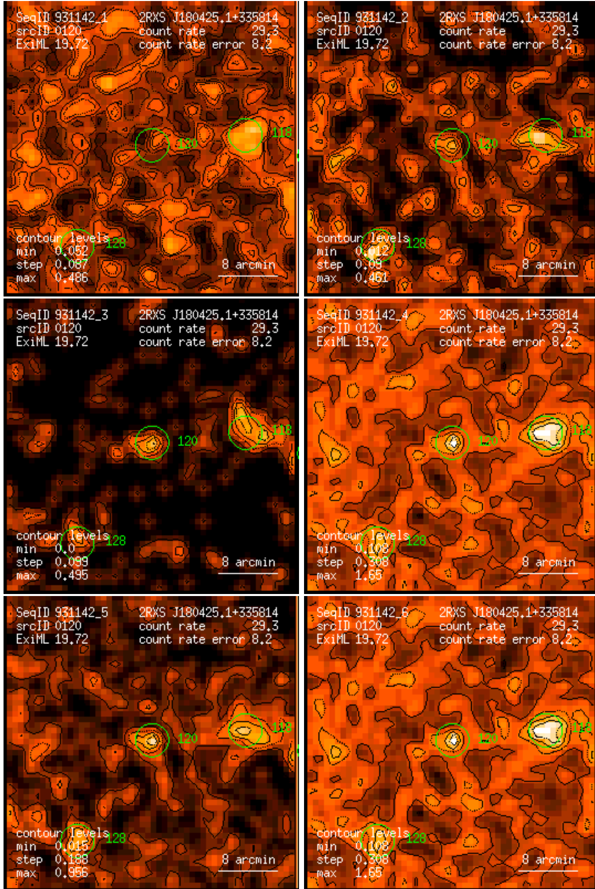
Figure 120: RASS 931142: detection 0120: band rate images, Gaussian filter: (1) PSPC channels 11 – 41, (2) 52 – 90, (3) 91 – 201, (4) 11 – 235, (5) 52 – 201, (6) 11 – 201. Broad band rates in counts/ks. Band rate contour levels in counts/ks/arcmin 2 .
