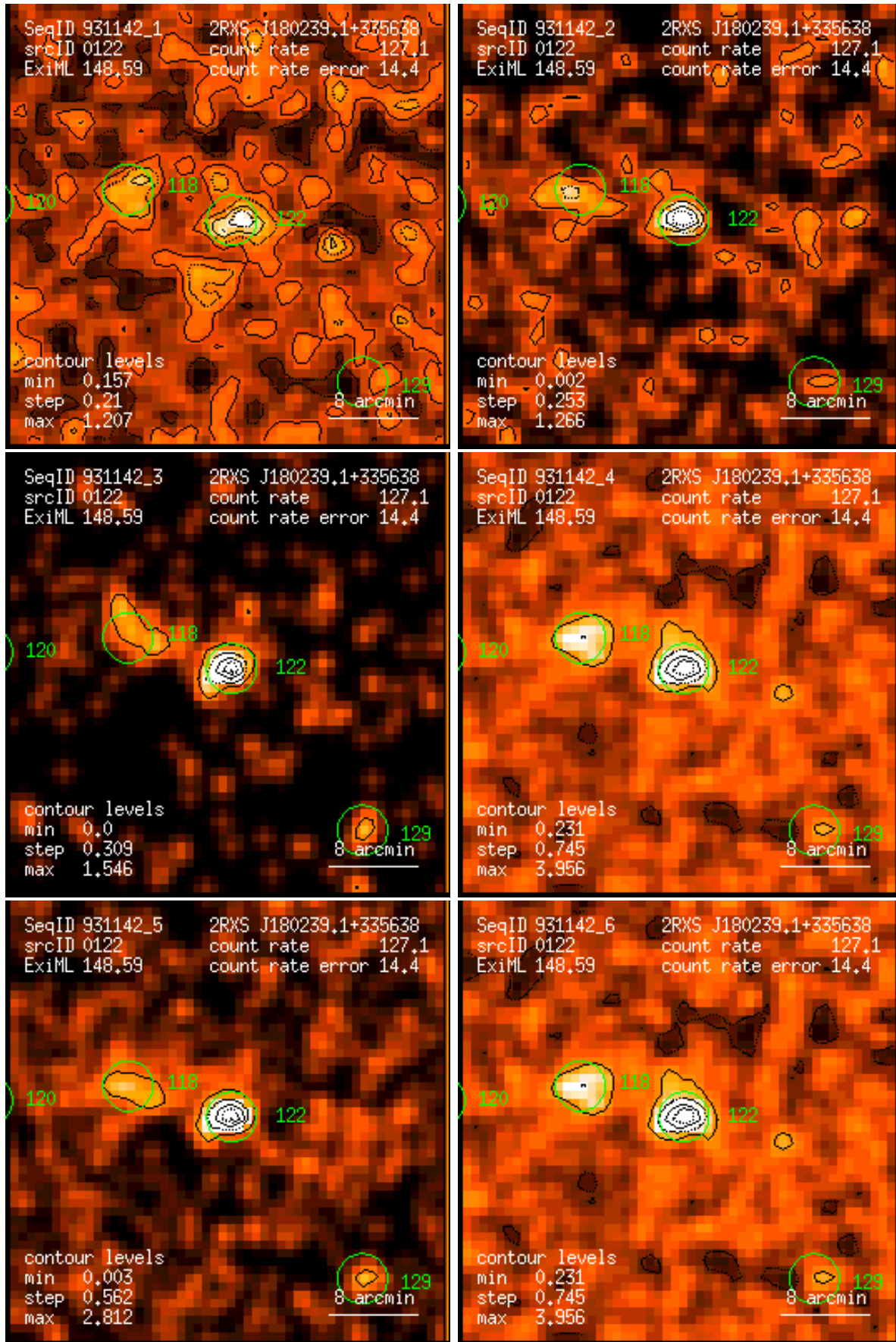
Figure 122: RASS 931142: detection 0122: band rate images, Gaussian filter: (1) PSPC channels 11 – 41, (2) 52 – 90, (3) 91 – 201, (4) 11 – 235, (5) 52 – 201, (6) 11 – 201. Broad band rates in counts/ks. Band rate contour levels in counts/ks/arcmin 2 .
