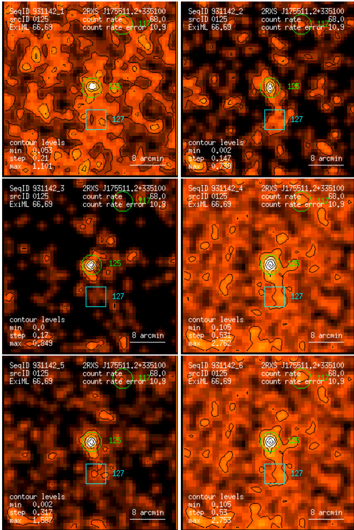
Figure 125: RASS 931142: detection 0125: band rate images, Gaussian filter: (1) PSPC channels 11 – 41, (2) 52 – 90, (3) 91 – 201, (4) 11 – 235, (5) 52 – 201, (6) 11 – 201. Broad band rates in counts/ks. Band rate contour levels in counts/ks/arcmin 2 .
