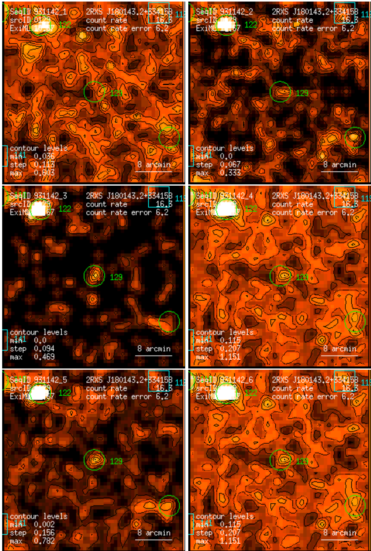
Figure 129: RASS 931142: detection 0129: band rate images, Gaussian filter: (1) PSPC channels 11 – 41, (2) 52 – 90, (3) 91 – 201, (4) 11 – 235, (5) 52 – 201, (6) 11 – 201. Broad band rates in counts/ks. Band rate contour levels in counts/ks/arcmin 2 .
