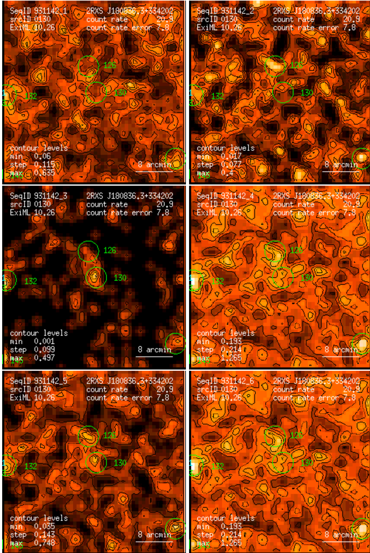
Figure 130: RASS 931142: detection 0130: band rate images, Gaussian filter: (1) PSPC channels 11 – 41, (2) 52 – 90, (3) 91 – 201, (4) 11 – 235, (5) 52 – 201, (6) 11 – 201. Broad band rates in counts/ks. Band rate contour levels in counts/ks/arcmin 2 .
