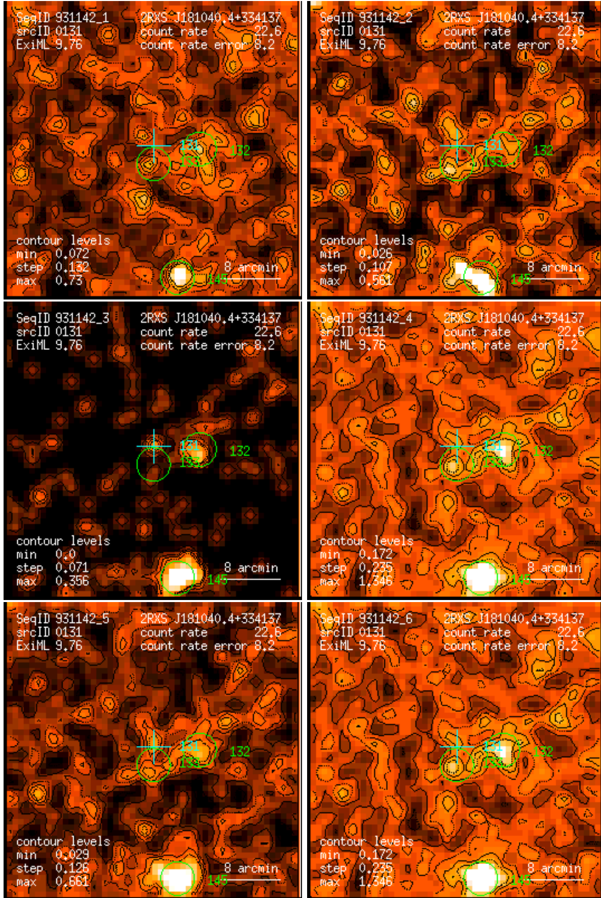
Figure 131: RASS 931142: detection 0131: band rate images, Gaussian filter: (1) PSPC channels 11 – 41, (2) 52 – 90, (3) 91 – 201, (4) 11 – 235, (5) 52 – 201, (6) 11 – 201. Broad band rates in counts/ks. Band rate contour levels in counts/ks/arcmin 2 .
