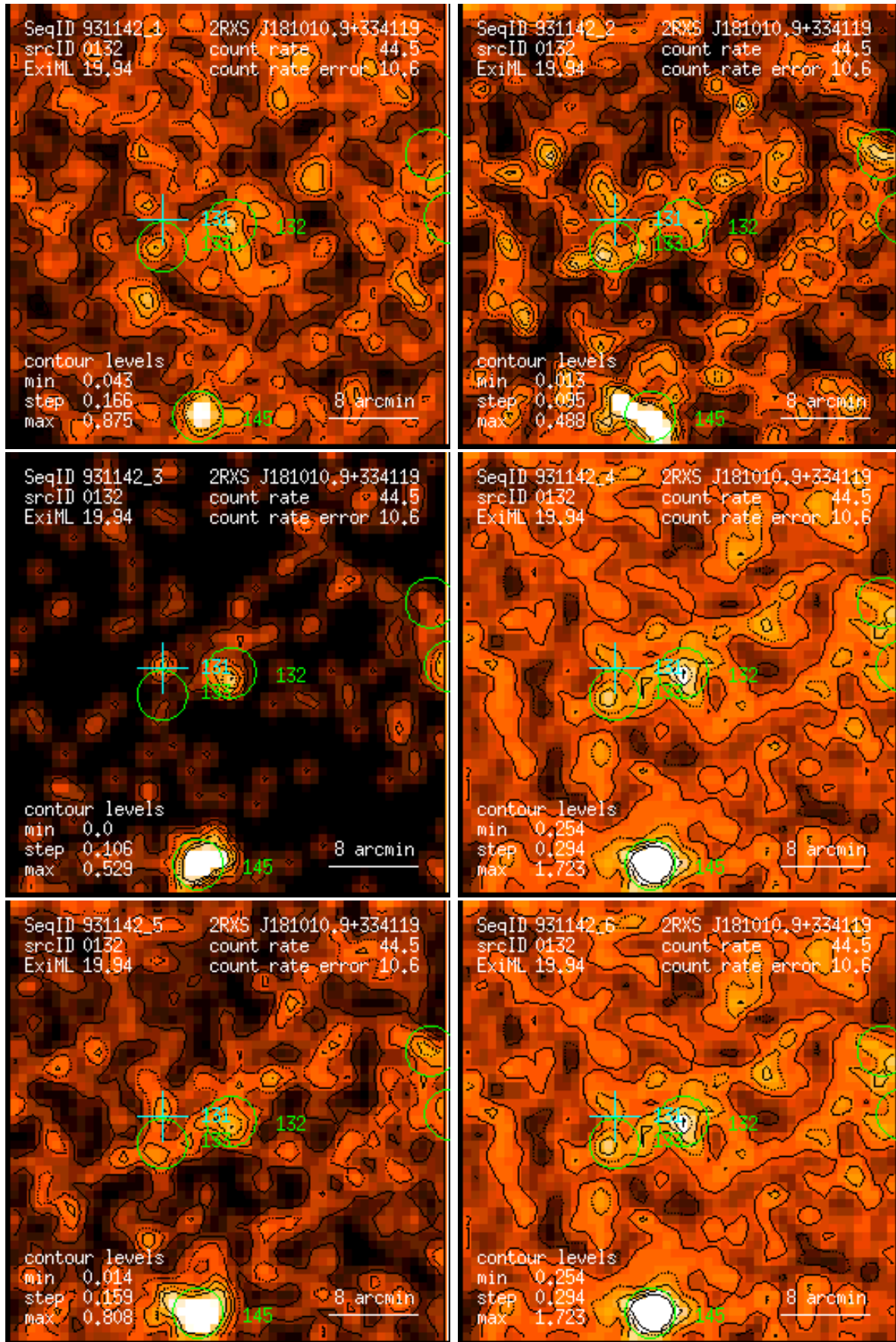
Figure 132: RASS 931142: detection 0132: band rate images, Gaussian filter: (1) PSPC channels 11 – 41, (2) 52 – 90, (3) 91 – 201, (4) 11 – 235, (5) 52 – 201, (6) 11 – 201. Broad band rates in counts/ks. Band rate contour levels in counts/ks/arcmin 2 .
