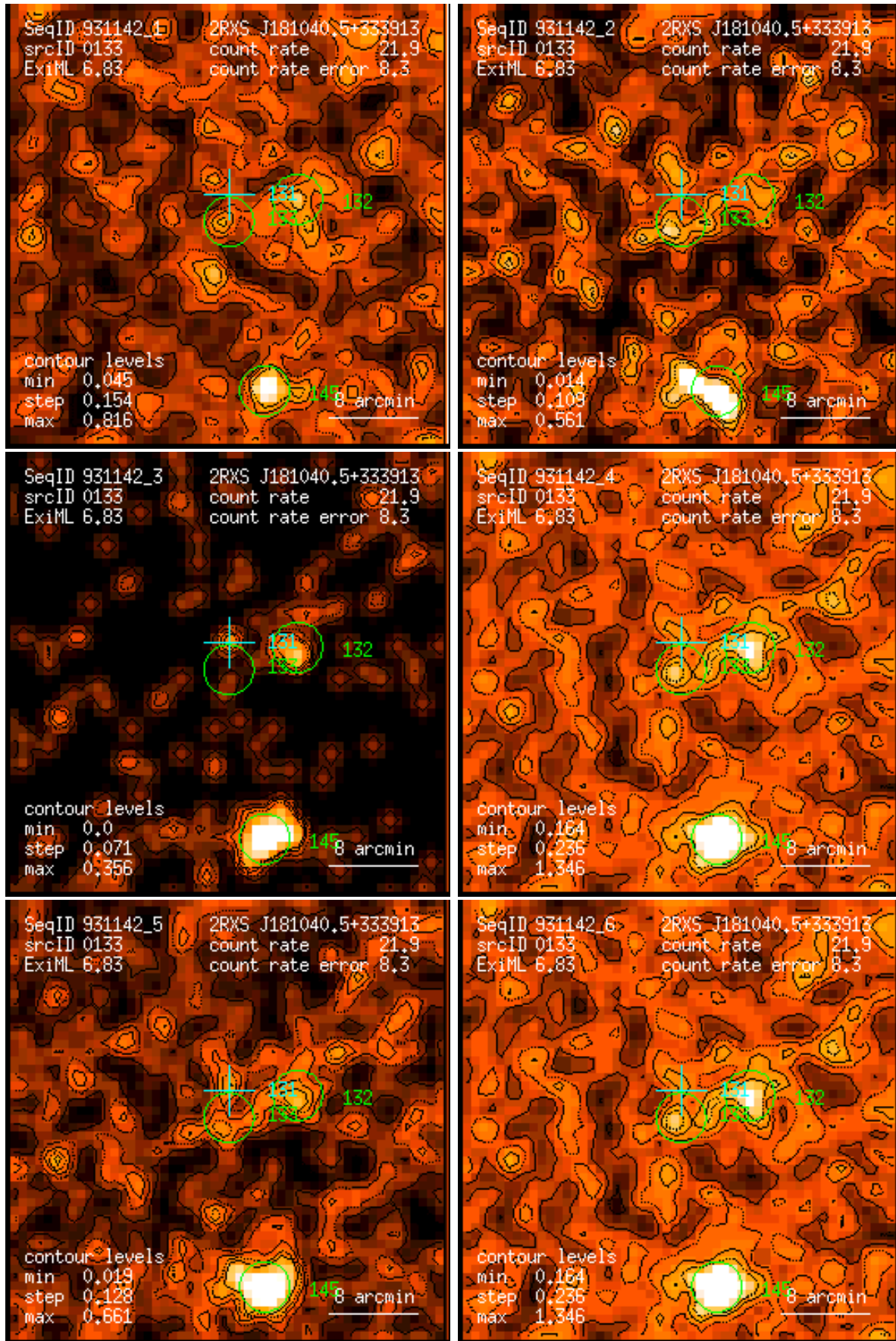
Figure 133: RASS 931142: detection 0133: band rate images, Gaussian filter: (1) PSPC channels 11 – 41, (2) 52 – 90, (3) 91 – 201, (4) 11 – 235, (5) 52 – 201, (6) 11 – 201. Broad band rates in counts/ks. Band rate contour levels in counts/ks/arcmin 2 .
