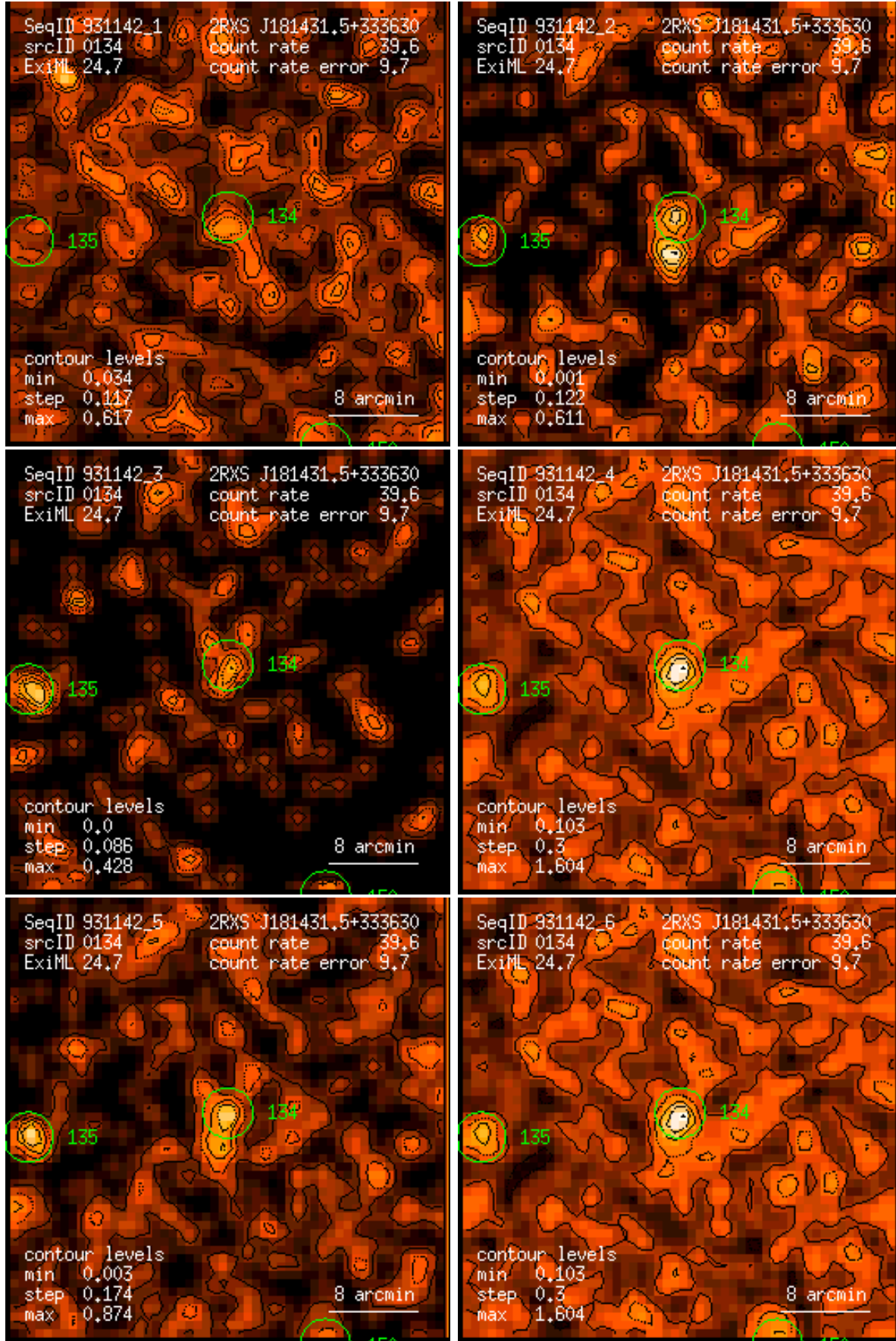
Figure 134: RASS 931142: detection 0134: band rate images, Gaussian filter: (1) PSPC channels 11 – 41, (2) 52 – 90, (3) 91 – 201, (4) 11 – 235, (5) 52 – 201, (6) 11 – 201. Broad band rates in counts/ks. Band rate contour levels in counts/ks/arcmin 2 .
