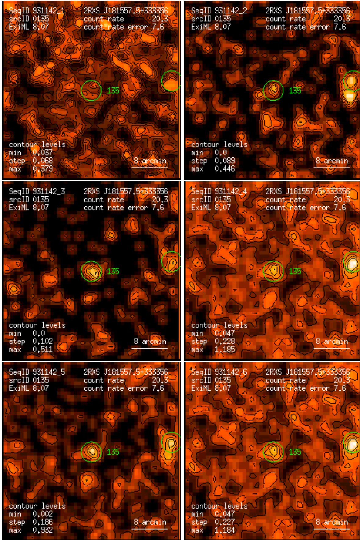
Figure 135: RASS 931142: detection 0135: band rate images, Gaussian filter: (1) PSPC channels 11 – 41, (2) 52 – 90, (3) 91 – 201, (4) 11 – 235, (5) 52 – 201, (6) 11 – 201. Broad band rates in counts/ks. Band rate contour levels in counts/ks/arcmin 2 .
