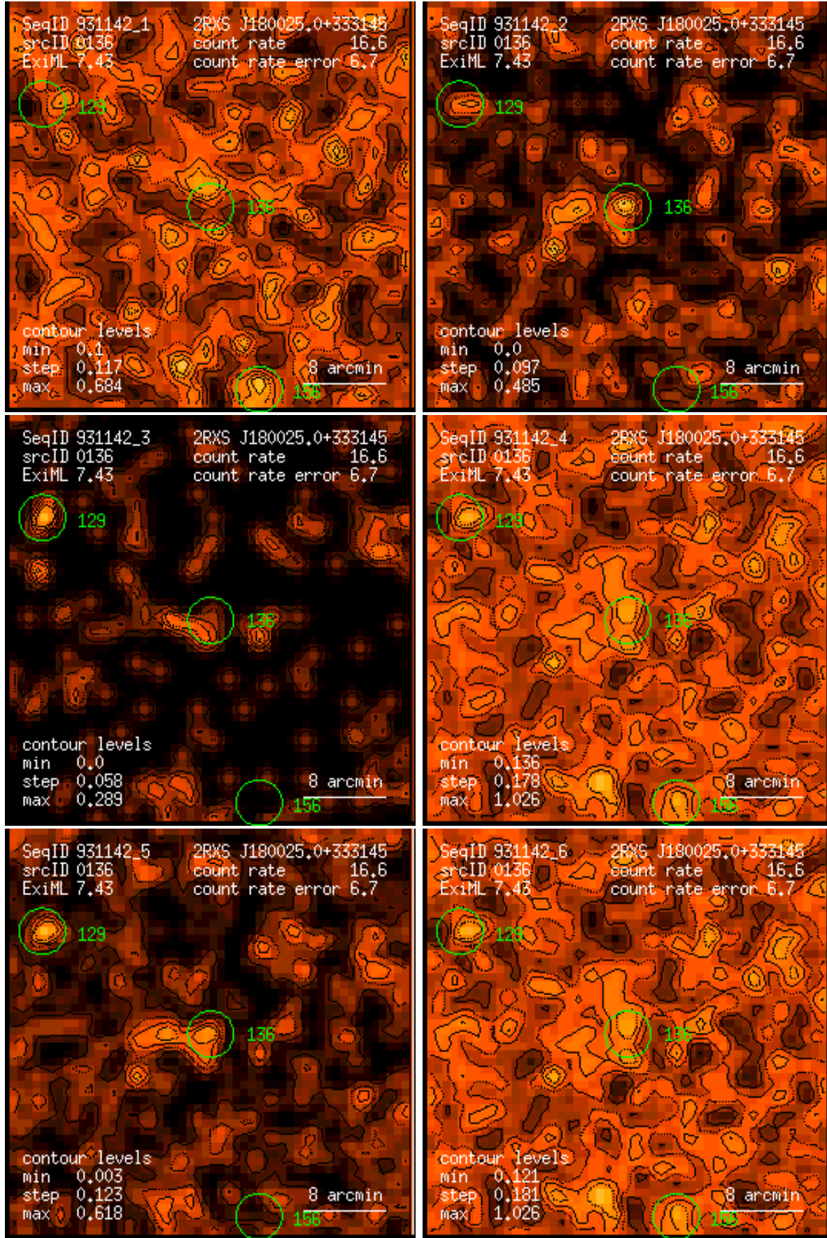
Figure 136: RASS 931142: detection 0136: band rate images, Gaussian filter: (1) PSPC channels 11 – 41, (2) 52 – 90, (3) 91 – 201, (4) 11 – 235, (5) 52 – 201, (6) 11 – 201. Broad band rates in counts/ks. Band rate contour levels in counts/ks/arcmin 2 .
