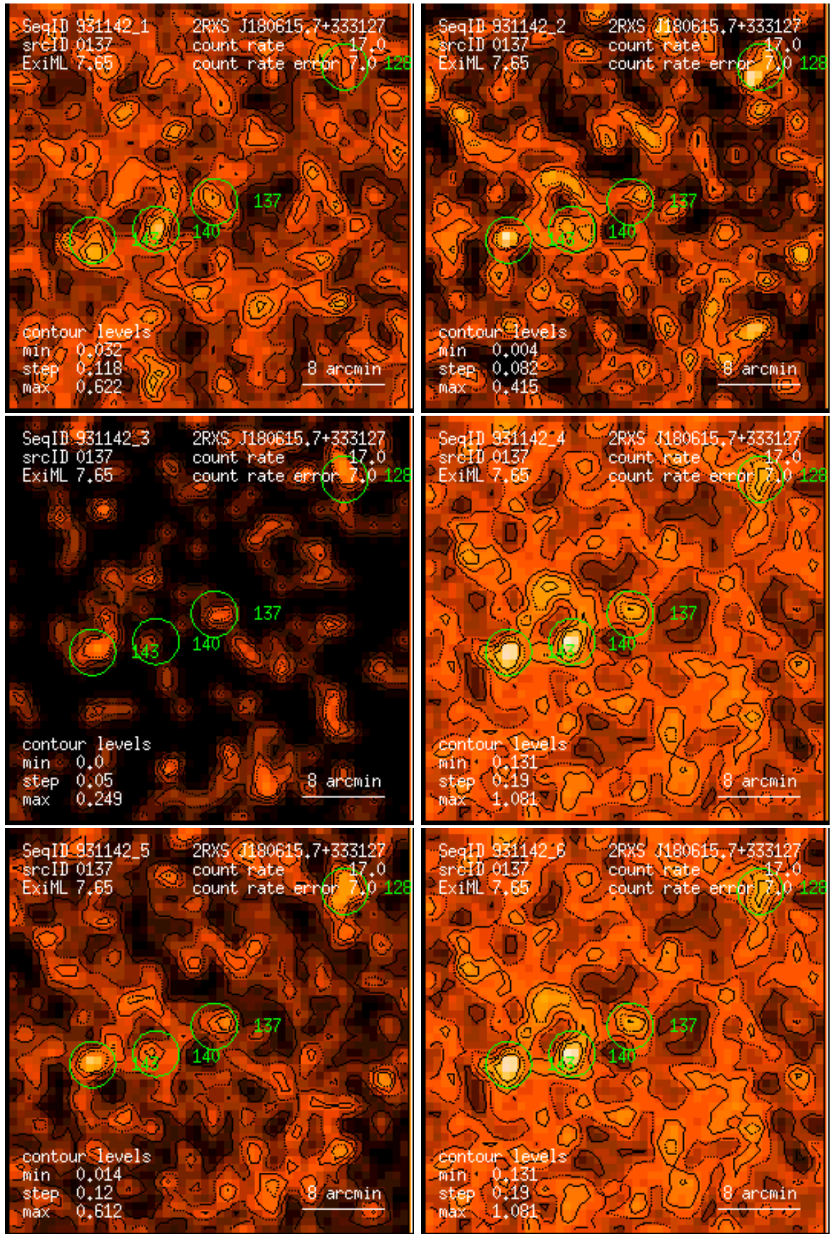
Figure 137: RASS 931142: detection 0137: band rate images, Gaussian filter: (1) PSPC channels 11 – 41, (2) 52 – 90, (3) 91 – 201, (4) 11 – 235, (5) 52 – 201, (6) 11 – 201. Broad band rates in counts/ks. Band rate contour levels in counts/ks/arcmin 2 .
