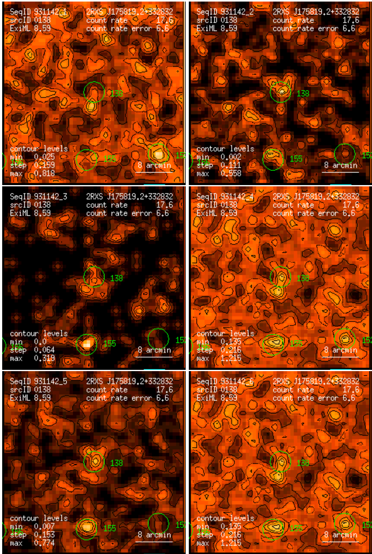
Figure 138: RASS 931142: detection 0138: band rate images, Gaussian filter: (1) PSPC channels 11 – 41, (2) 52 – 90, (3) 91 – 201, (4) 11 – 235, (5) 52 – 201, (6) 11 – 201. Broad band rates in counts/ks. Band rate contour levels in counts/ks/arcmin 2 .
