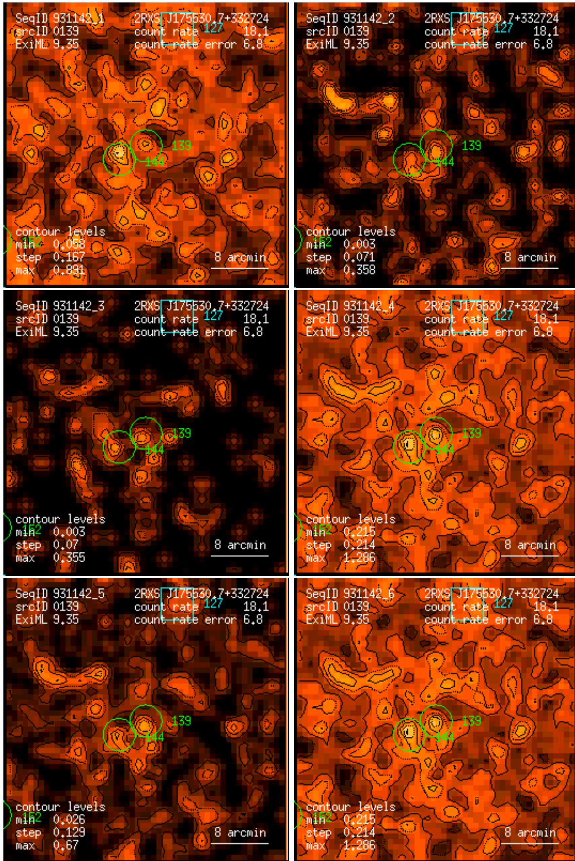
Figure 139: RASS 931142: detection 0139: band rate images, Gaussian filter: (1) PSPC channels 11 – 41, (2) 52 – 90, (3) 91 – 201, (4) 11 – 235, (5) 52 – 201, (6) 11 – 201. Broad band rates in counts/ks. Band rate contour levels in counts/ks/arcmin 2 .
