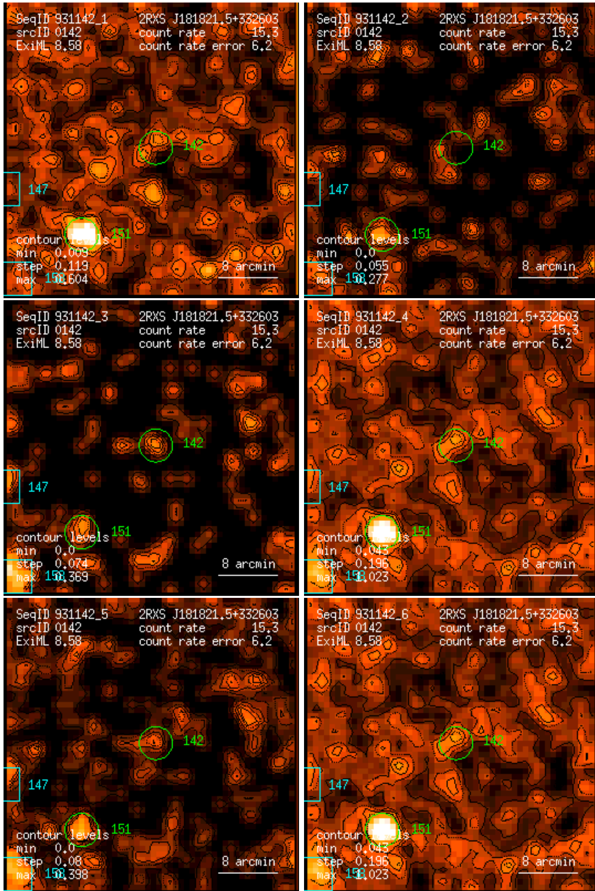
Figure 142: RASS 931142: detection 0142: band rate images, Gaussian filter: (1) PSPC channels 11 – 41, (2) 52 – 90, (3) 91 – 201, (4) 11 – 235, (5) 52 – 201, (6) 11 – 201. Broad band rates in counts/ks. Band rate contour levels in counts/ks/arcmin 2 .
