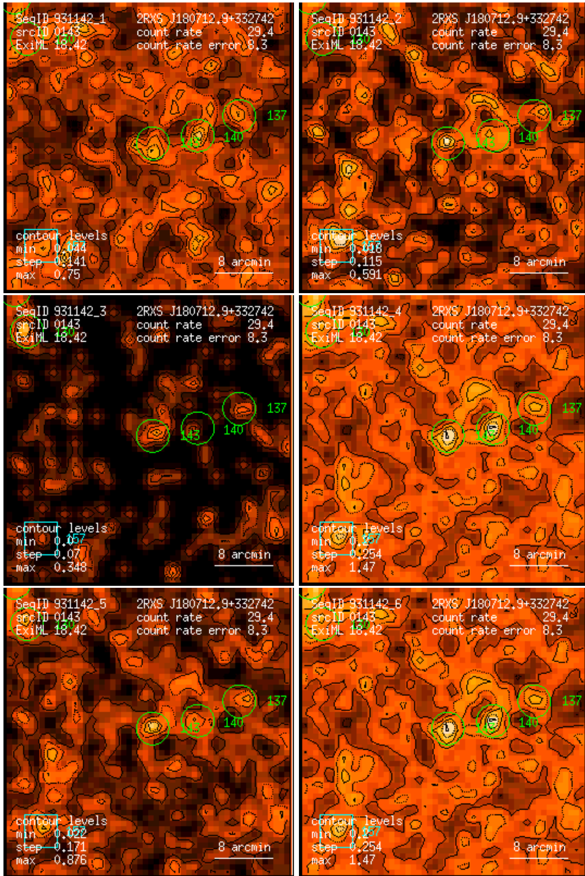
Figure 143: RASS 931142: detection 0143: band rate images, Gaussian filter: (1) PSPC channels 11 – 41, (2) 52 – 90, (3) 91 – 201, (4) 11 – 235, (5) 52 – 201, (6) 11 – 201. Broad band rates in counts/ks. Band rate contour levels in counts/ks/arcmin 2 .
