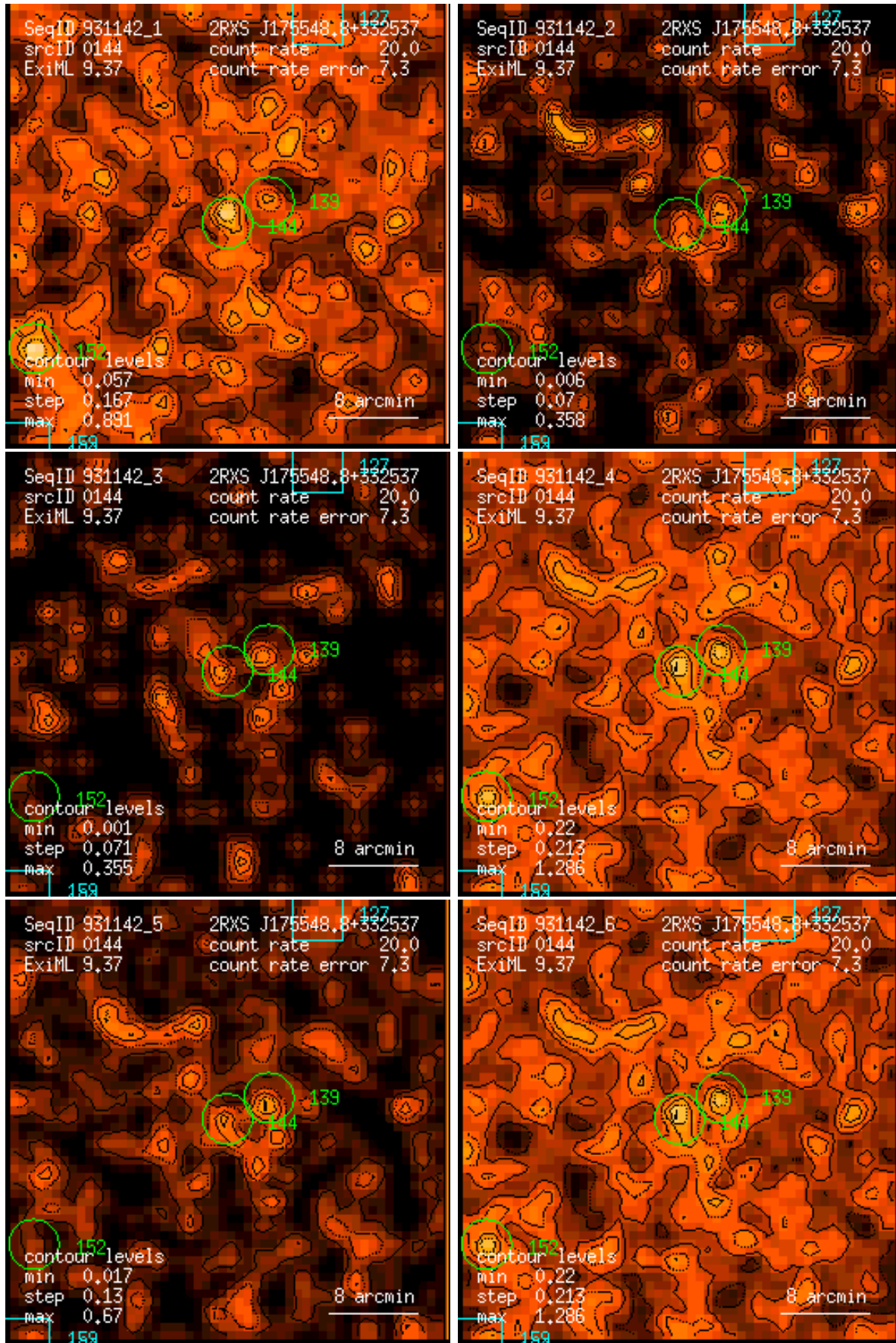
Figure 144: RASS 931142: detection 0144: band rate images, Gaussian filter: (1) PSPC channels 11 – 41, (2) 52 – 90, (3) 91 – 201, (4) 11 – 235, (5) 52 – 201, (6) 11 – 201. Broad band rates in counts/ks. Band rate contour levels in counts/ks/arcmin 2 .
