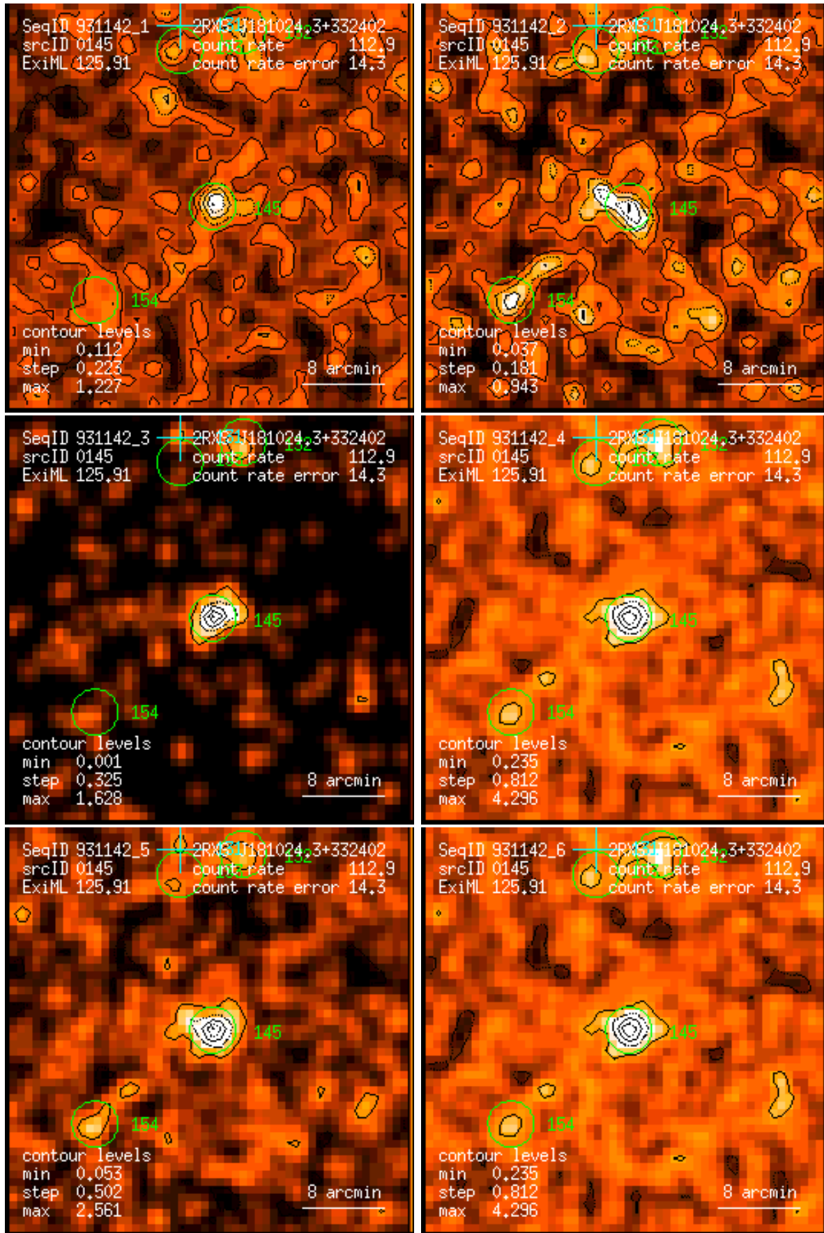
Figure 145: RASS 931142: detection 0145: band rate images, Gaussian filter: (1) PSPC channels 11 – 41, (2) 52 – 90, (3) 91 – 201, (4) 11 – 235, (5) 52 – 201, (6) 11 – 201. Broad band rates in counts/ks. Band rate contour levels in counts/ks/arcmin 2 .
