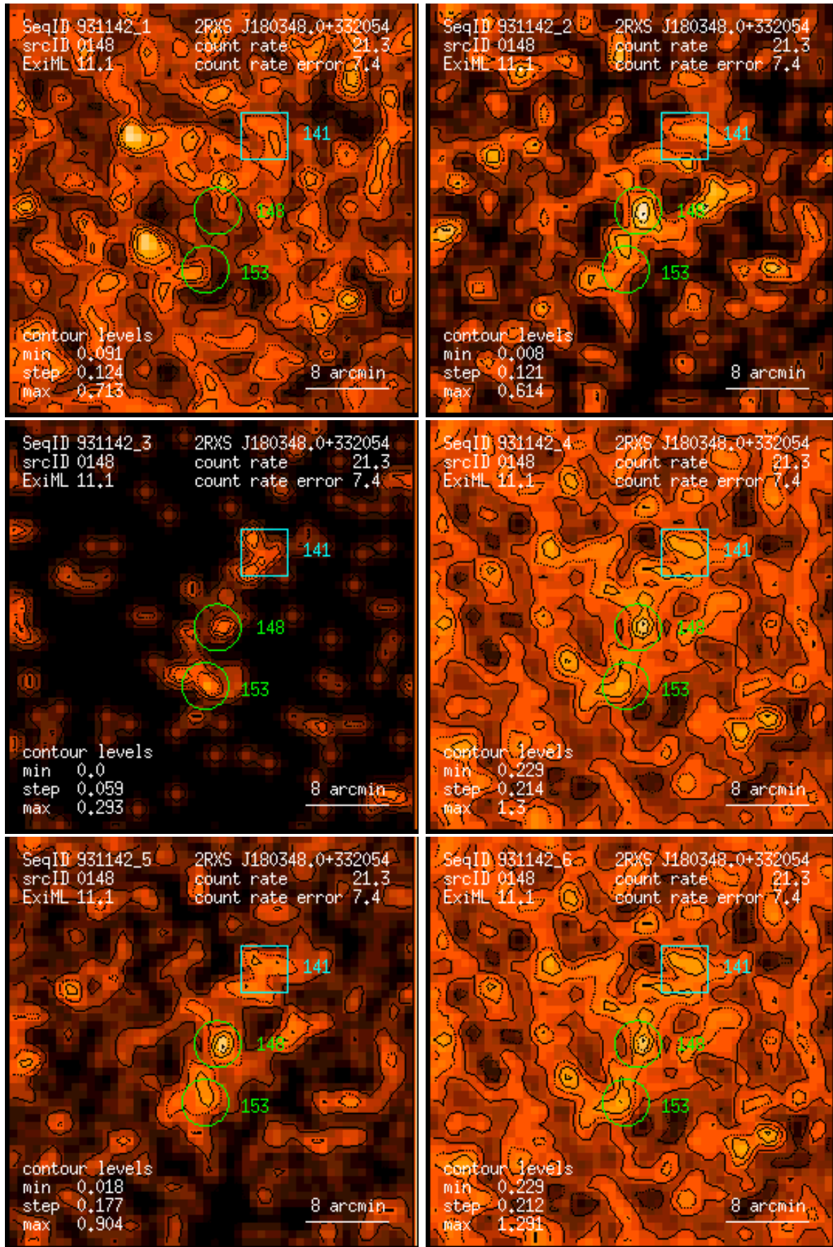
Figure 148: RASS 931142: detection 0148: band rate images, Gaussian filter: (1) PSPC channels 11 – 41, (2) 52 – 90, (3) 91 – 201, (4) 11 – 235, (5) 52 – 201, (6) 11 – 201. Broad band rates in counts/ks. Band rate contour levels in counts/ks/arcmin 2 .
