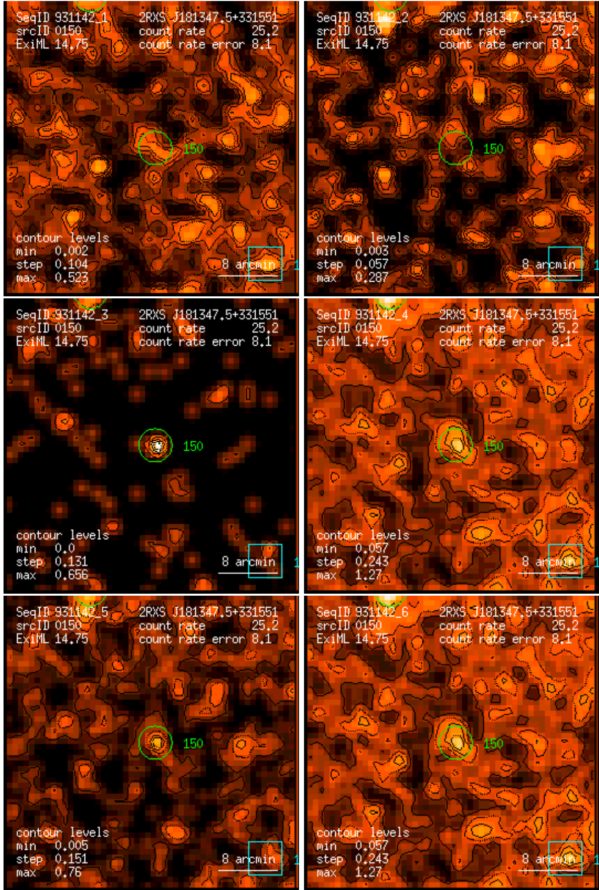
Figure 150: RASS 931142: detection 0150: band rate images, Gaussian filter: (1) PSPC channels 11 – 41, (2) 52 – 90, (3) 91 – 201, (4) 11 – 235, (5) 52 – 201, (6) 11 – 201. Broad band rates in counts/ks. Band rate contour levels in counts/ks/arcmin 2 .
