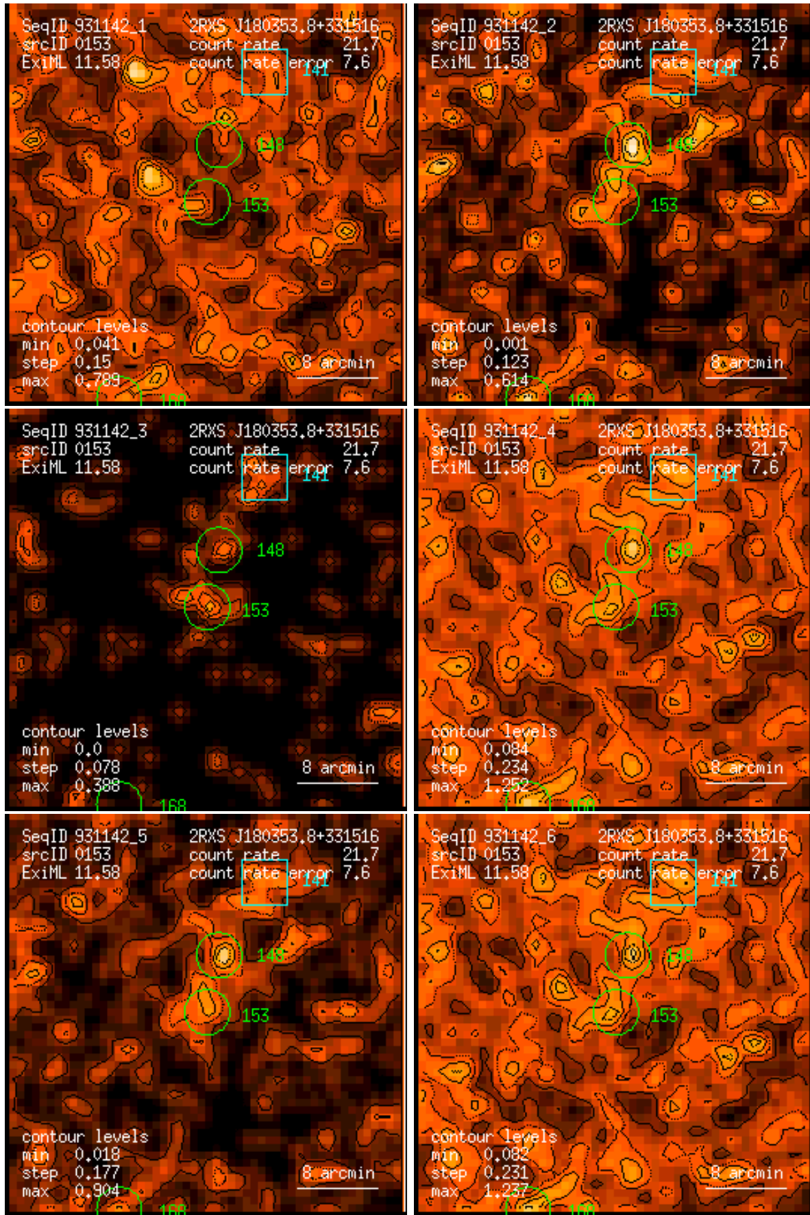
Figure 153: RASS 931142: detection 0153: band rate images, Gaussian filter: (1) PSPC channels 11 – 41, (2) 52 – 90, (3) 91 – 201, (4) 11 – 235, (5) 52 – 201, (6) 11 – 201. Broad band rates in counts/ks. Band rate contour levels in counts/ks/arcmin 2 .
