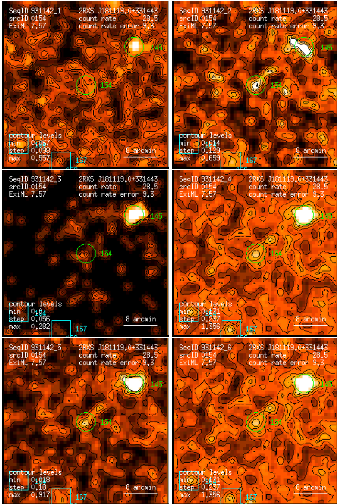
Figure 154: RASS 931142: detection 0154: band rate images, Gaussian filter: (1) PSPC channels 11 – 41, (2) 52 – 90, (3) 91 – 201, (4) 11 – 235, (5) 52 – 201, (6) 11 – 201. Broad band rates in counts/ks. Band rate contour levels in counts/ks/arcmin 2 .
