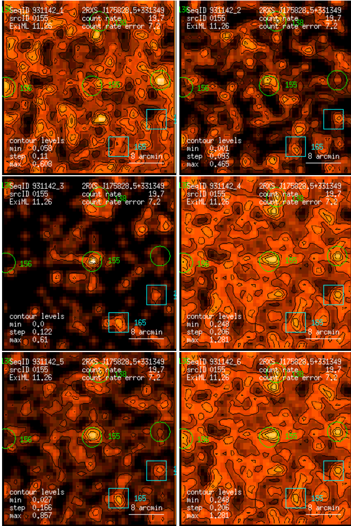
Figure 155: RASS 931142: detection 0155: band rate images, Gaussian filter: (1) PSPC channels 11 – 41, (2) 52 – 90, (3) 91 – 201, (4) 11 – 235, (5) 52 – 201, (6) 11 – 201. Broad band rates in counts/ks. Band rate contour levels in counts/ks/arcmin 2 .
