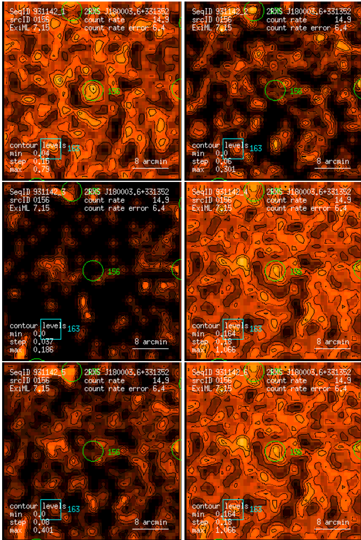
Figure 156: RASS 931142: detection 0156: band rate images, Gaussian filter: (1) PSPC channels 11 – 41, (2) 52 – 90, (3) 91 – 201, (4) 11 – 235, (5) 52 – 201, (6) 11 – 201. Broad band rates in counts/ks. Band rate contour levels in counts/ks/arcmin 2 .
